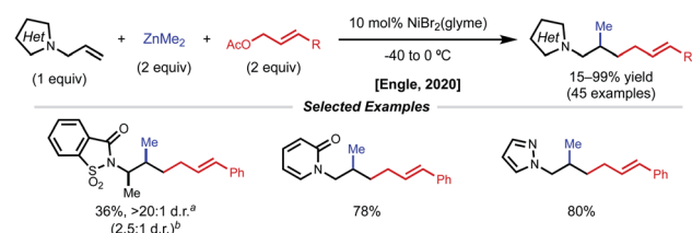
Fig. 15 1,2-Allylmethylation of N -allyl heterocycles.
