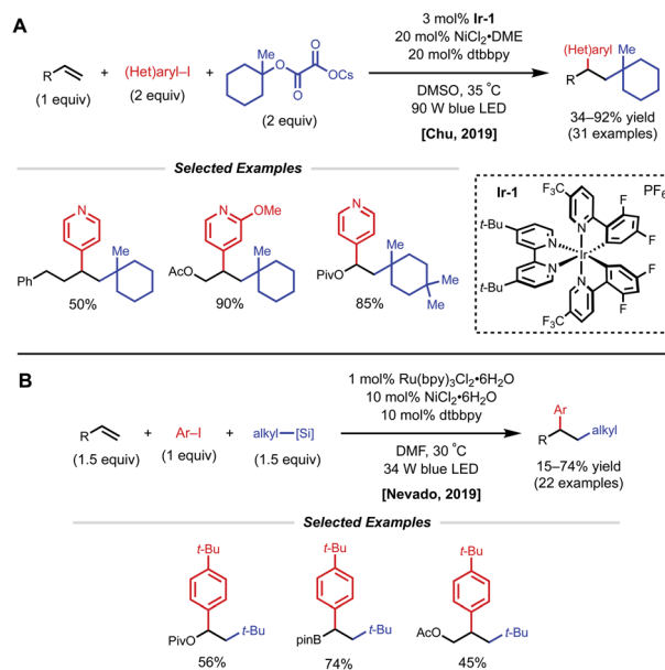
Fig. 17 Photocatalytic 1,2-arylalkenylation of alkenes reported by (A) Chu and coworkers and (B) Nevado and coworkers.
