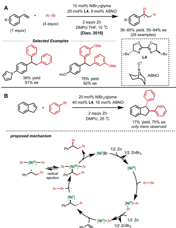
Fig. 7 (A) Asymmetric reductive 1,2-homodarylation of vinyl arenes. (B) Key mechanistic experiment and proposed catalytic cycle.
