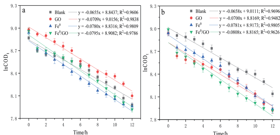
Fig. 4 Fitted first-order kinetics curves: (a) 30 °C and (b) 50 °C.
