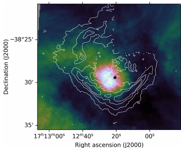
Fig. 3. Chandra diffuse x-ray emission toward RCW 120. The color scale ranges from 0 to 1.1 \times 10^{-9} photons \text{cm}^{-2} \text{s}^{-1} \text{arc sec}^{-2} . The contours are of integrated [CII] intensity, scaled from 40 to 160 K km/s in 40 K km/s increments, and the location of the ionizing source is marked by the black star. There is strong diffuse x-ray emission within the bubble, which is breaching the PDR toward the northeast.
