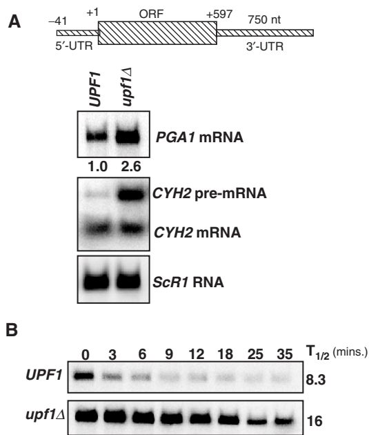
Figure 2. The PGAI mRNA is degraded by the NMD pathway. PGAI mRNA schematic and northern analysis of the PGAI mRNA accumulation (A), and half-lives (B) in wild-type ( UPF1 ) and NMD mutant ( upf1Δ ) yeast cells. The mRNA accumulations were measured using total RNA isolated from yeast strain W303a [ UPF1 (24)] and AAY320 [ upf1-Δ2 (17)]. CYH2 and ScR1 are controls (25,26). CYH2 is a control for the NMD phenotype of the yeast strains. The CYH2 probe detects both the CYH2 pre-mRNA and mRNA. CYH2 pre-mRNA is inefficiently spliced. Consequently, a significant amount of the pre-mRNA is transported to the cytoplasm where it is targeted for NMD by an in-frame stop codon within the intron. In contrast, CYH2 mRNA is not degraded by NMD. ScR1 is an RNA polymerase III transcript that is not degraded by NMD. It was used as a loading control. mRNA half-lives were determined using total mRNA isolated from yeast strains AAY334 [ UPF1 (17)] and AAY335 [ upf1-Δ2 (17)] at time points following transcriptional arrest. The mRNA half-lives ( T_{1/2} ) are an average of at least three independent experiments.
