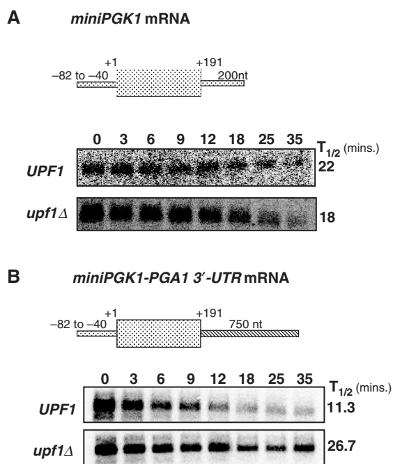
Figure 3. The long 3'-UTR of PGAI mRNA is sufficient to target a NMD-insensitive mRNA to NMD. The mRNA schematics and northern blot analysis of miniPGK1 (A), and miniPGK1-PGAI 3'-UTR (B) mRNAs. The mRNA half-lives ( T_{1/2} ) were determined as described in Figure 2 and are shown to the right of the phosphorimages. They are an average of three independent experiments, with the exception of the half-life for the miniPGK1 mRNA in the upf1Δ strain (A), which is an average of two experiments. The miniPGK1 mRNA half-lives measured here are consistent with the half-lives determined for this mRNA by Hagan et al. (28).
