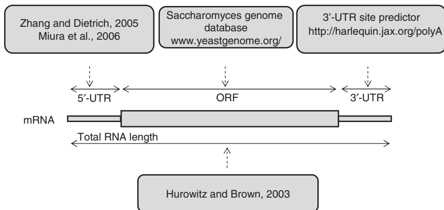
Figure 1. Strategy used to predict the primary sequence of S. cerevisiae mRNAs. The 5'-UTR length was determined from the location of the transcription start site [Zhang and Dietrich, 2005 (20); http://data.cgt.duke.edu/5sage.php ; Miura et al. , 2006 (19); http://yeast.utgenome.org/ ]. The ORF lengths were obtained from the SGD ( www.yeastgenome.org/ ). The mRNA 3'-processing Site Predictor [Graber et al. , 2002 (21); http://harlequin.jax.org/polyA/ ] was used to predict the lengths of the 3'-UTRs. The 3'-UTR lengths were determined experimentally by 3'-RACE. Virtual northern transcript lengths were from a genome-wide study measuring transcript lengths [Hurowitz and Brown, 2003 (18); http://microarray-pubs.stanford.edu/vnorth/ ].
