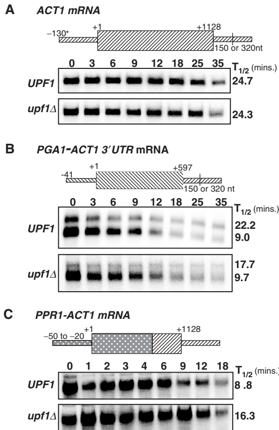
Figure 4. Replacement of the long 3'-UTR of PGA1 mRNA with a short 3'-UTR protects this mRNA from decay by the NMD pathway. The mRNA schematics and northern blot analysis of ACT1 (A), PGA1-ACT1 3'-UTR (B), and PPR1-ACT1 (C) mRNAs. The mRNA half-lives were determined as described in Figure 2 and are shown to the right of the PhosphorImages.
