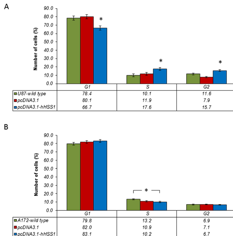
Figure 5 Effect of hHSS1 on cell cycle phases for glioma cells. Cell cycle analysis in A ) U87 cells and B ) A172 cells. Cell cycle analysis was performed by propidium iodide staining followed by flow cytometry using day 4 and 5 from a U87 and A172 cell growth curve, respectively. Columns represent the mean percentage of cells in each phase of the cell cycle \pm SEM (n = 2), P < 0.05 , one way ANOVA with post hoc pairwise Tukey test.
