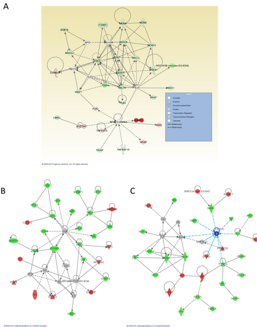
Figure 1 Top molecular networks of genes up- and down-regulated in U87 and A172 cells overexpressing hHSS1 . Network of genes based on connectivity identified by IPA analysis. A) Top gene network of U87 cells depicting genes involved in cell cycle, cell death, DNA replication, recombination and repair. ANKRD1 was the most up-regulated gene. Many genes with a direct and indirect relationship with E2F gene were down-regulated by HSS1 . B) Top gene network of A172- hHSS1 C#7 showing genes involved in cell cycle, cellular assembly and organization, DNA replication, recombination and repair. Several genes down-regulated by hHSS1 in A172 C#7 cells are target genes regulated by VEGF . C) Top gene network of A172- hHSS1 C#8 showing genes involved in tissue morphology and cellular development. Some of the hHSS1 modulated genes in A172 C#8 cells are responsible for ERK regulation. Different shapes of the nodes (genes/gene products) represent the functional classes of the gene products and the lines represent the biological relationships between the nodes. The length of an edge reflects the evidence in the literature supporting that node-to-node relationship. The intensity of the node color indicates the degree of up- (red) or down-regulation (green) of the respective gene. Gray represents a gene related to the others that did not meet the cutoff criteria. A solid line without arrow indicates protein-protein interaction. Arrows indicate the direction of action (either with or without binding) of one gene to another.
