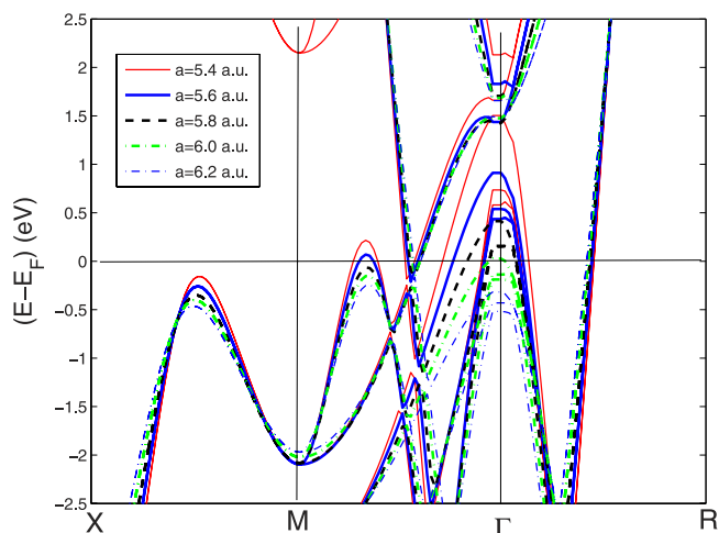
Figure 9. The band structure for \text{H}_3\text{S} along X\text{-M-}\Gamma\text{-R} for a for the simple cubic double cell (sc BZ) with the lattice parameter changing between 5.4 and 6.2 a.u.
