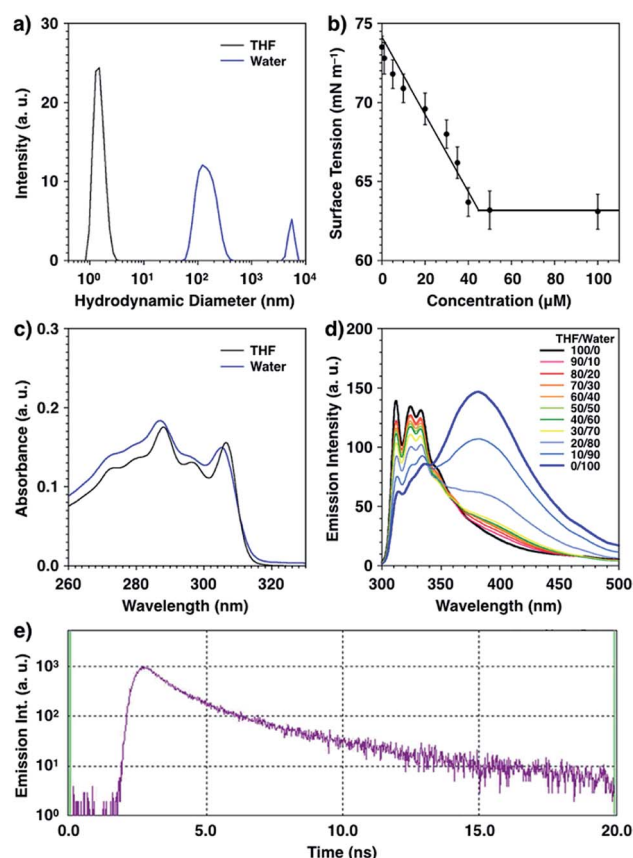
Fig. 1 (a) DLS size distribution profiles of bola -AkDPA in THF (black) and water (blue) at 50 \mu\text{M} at 20 °C. (b) Concentration-dependent surface tension changes of bola -AkDPA in water at 20 °C. (c) UV absorption spectra of bola -AkDPA in THF (black) and water (blue) at 50 \mu\text{M} at 20 °C. (d) Fluorescence spectra of bola -AkDPA in mixtures of THF and water at varying ratios at 50 \mu\text{M} at 20 °C. Excitation: 288 nm. (e) Fluorescence intensity decay profile of bola -AkDPA in water at 20 °C. Excitation: 280 nm, emission: 380 nm. [\textit{bola}\text{-AkDPA}] = 50 \mu\text{M} .
