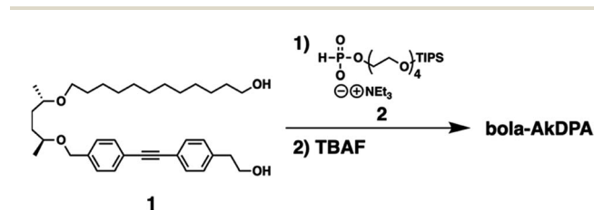
Scheme 2 Synthetic scheme of bola-AkDPA.
