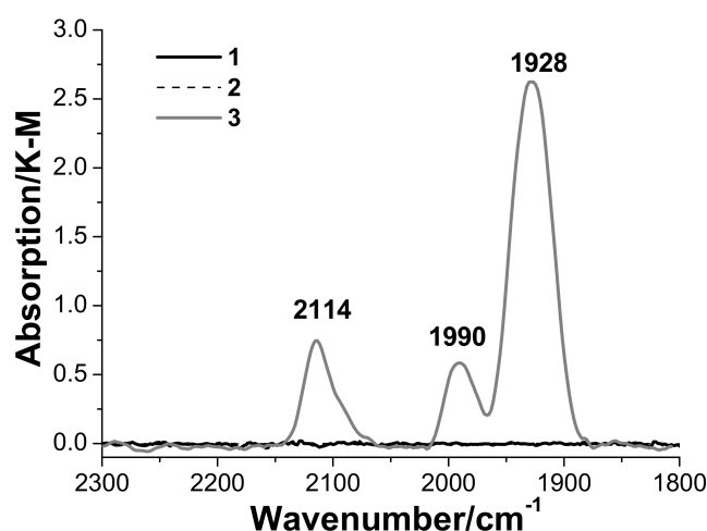
Figure 7. DRIFT spectra of samples 1 (Al 2 O 3 ), 2 (CuCl 2 /Al 2 O 3 ) and 3 (PdCl 2 –CuCl 2 / \gamma -Al 2 O 3 ) at an equilibrium CO pressure of 20 Torr and room temperature (the intensity scale is expressed in Kubelka-Munk units).
