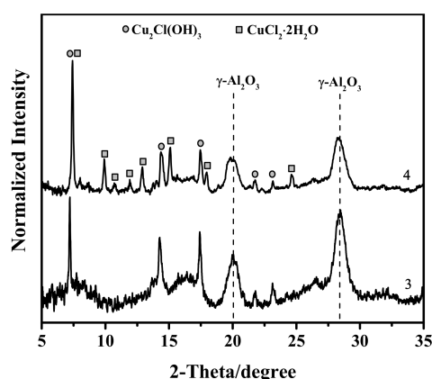
Figure 2. X-ray diffraction patterns of catalysts 3 ( \text{PdCl}_2\text{-CuCl}_2/\gamma\text{-Al}_2\text{O}_3 , 3.5 wt % Cu, 1.5 wt % Pd) and 4 ( \text{PdCl}_2\text{-CuCl}_2/\gamma\text{-Al}_2\text{O}_3 , 17.5 wt % Cu, 1.5 wt % Pd).
