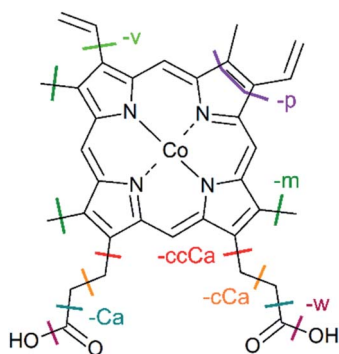
Fig. 4 Structure of \text{CoPPIX}^+ . The indicated bond cleavages lead to the observed fragments in Fig. 2 and in Fig. 3.
