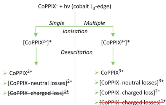
Scheme 1 Possible photo products upon single and multiple ionisation after resonant cobalt 2p inner-shell excitation of CoPPIX + at 780.5 eV at the cobalt L_{3-} -edge. Photo products which are not observed in the mass spectrum in Fig. 2 and in ESI-2† are crossed out in red.
