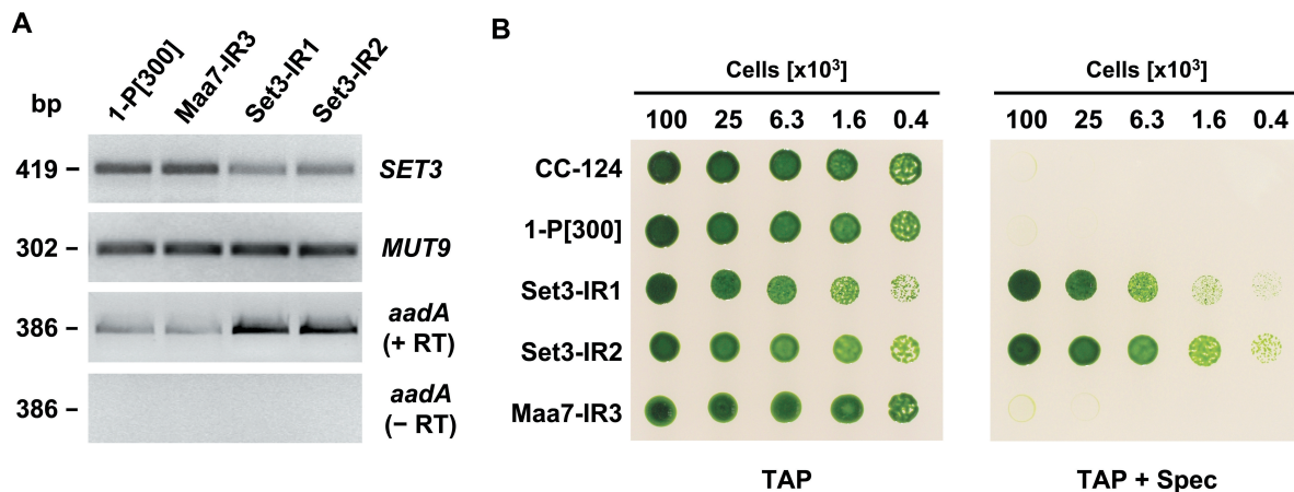
Figure 2. Suppression of SET3 expression and reactivation of RbcS2:aadA:RbcS2 transgenes in Set3-IR strains. (A) RT-PCR analysis of SET3 and RbcS2:aadA:RbcS2 ( aadA ) expression in the indicated strains. Amplification of MUT9 (encoding a Ser/Thr protein kinase) transcripts was used as a control for equivalent RNA input and efficiency of the RT-PCR reactions. (B) Growth and survival of the indicated strains on medium with (TAP + Spec) or without (TAP) spectinomycin. Strains: CC-124, wild-type strain; 1-P[300], silenced parental strain; Maa7-IR3, 1-P[300] transformant expressing dsRNA complementary to the MAA7 gene; Set3-IR1 and Set3-IR2, 1-P[300] transformants expressing dsRNA complementary to SET3 .
