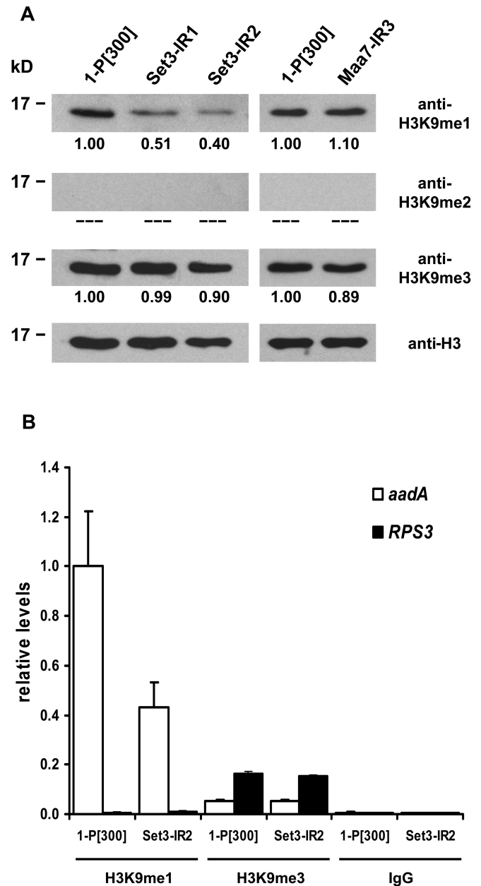
Figure 4. Monomethyl H3K9 is dependent on SET3p and is associated with the transcriptionally silenced RbcS2:aadA:RbcS2 transgenes. (A) Immunoblot analysis of in vivo H3K9 methylation states. Partially purified chromatin proteins from the indicated strains were separated by SDS-PAGE, transferred to nitrocellulose and probed with antibodies raised against mono-, di- or trimethyl H3K9. Sample loading was calibrated based on immunoblots with an anti-H3, modification-insensitive antibody. Numbers below the panels indicate relative levels of a specific histone modification normalized to the histone H3 amount. (B) Association of mono- and trimethyl H3K9 with the silent RbcS2:aadA:RbcS2 transgenes and the transcriptionally active RPS3 gene. Sequential ChIP assays were performed on TAP-grown cells of the indicated strains using an antibody against histone H3, and then antibodies against monomethyl H3K9, trimethyl H3K9 or rabbit IgG (negative control). Immunoprecipitated DNA was examined by real-time PCR. For illustration purposes, enrichment was calculated relative to the level of monomethyl H3K9 associated with the RbcS2:aadA:RbcS2 transgenes in the 1-P[300] strain. Results represent the mean \pm SD of three independent experiments.
