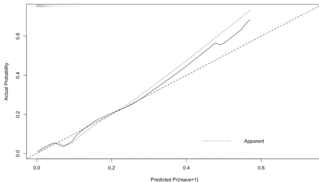
Figure 5. Calibration plot showing relation between the observed and predicted outcome.
