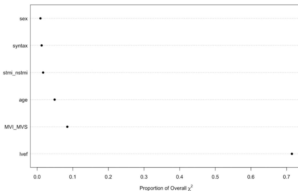
Figure 2. Importance of individual predictors. The importance of each predictor in our model was calculated as the proportion of the explainable outcome variation contributed by each predictor (partial \chi^2 value for each predictor divided by the model’s total \chi^2 ).
