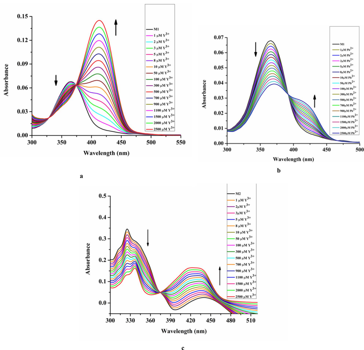
Fig. 2 UV-vis titration: M1 (20 \mu\text{M} ) vs. [M^{n+}] where M^n = Y^{3+} [0–2500 \mu\text{M} ] (a) and Pb^{2+} [0–2500 \mu\text{M} ] (b); M2 (20 \mu\text{M} ) vs. [Y^{3+}] [0–2500 \mu\text{M} ] (c) HEPES buffered EtOH/ H_2O (4/1, v/v, pH 7.4).
