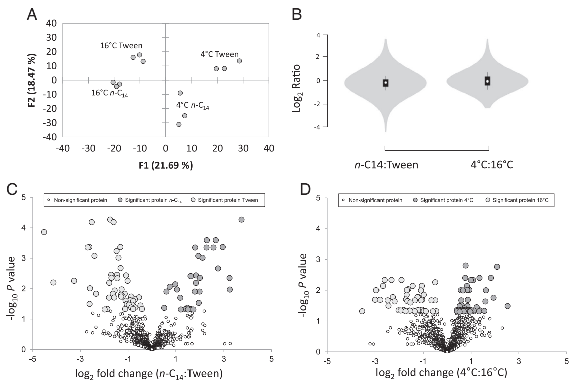
Fig. 1. A. Principle component analysis of replicate Oleispira antarctica RB-8 proteomes during growth on tetradecane ( n\text{-C}_{14} ) and the non-hydrocarbon control Tween 80 (Tween) at 4°C and 16°C based on normalized spectral counts for proteins. B. Violin plots of normalized LC–MS/MS spectral counts showing the distribution of detected proteins in O. antarctica RB-8 during growth on different substrates; n\text{-C}_{14} versus Tween (left; n\text{-C}_{14} :Tween); and different temperature; 4°C versus 16°C (right; 4°C:16°C). C and D. Volcano plots of normalized LC–MS/MS spectral counts comparing O. antarctica RB-8 protein abundance during growth on different substrates; n\text{-C}_{14} versus Tween (left; n\text{-C}_{14} : Tween) and different temperatures; 4°C versus 16°C (right; 4°C:16°C). Larger data points (light and dark grey) represent differentially expressed proteins with P -values below 0.05.
