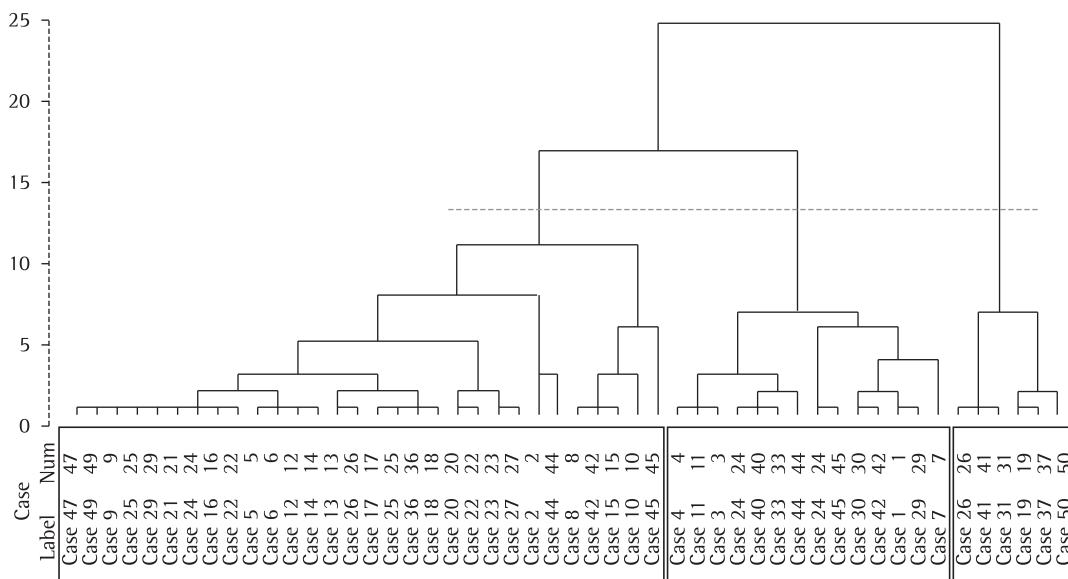
Figure 1 - Dendrogram obtained by using the farthest neighbor method. Clusters were formed on the basis of the distances between individual magnitudes of symptoms.
