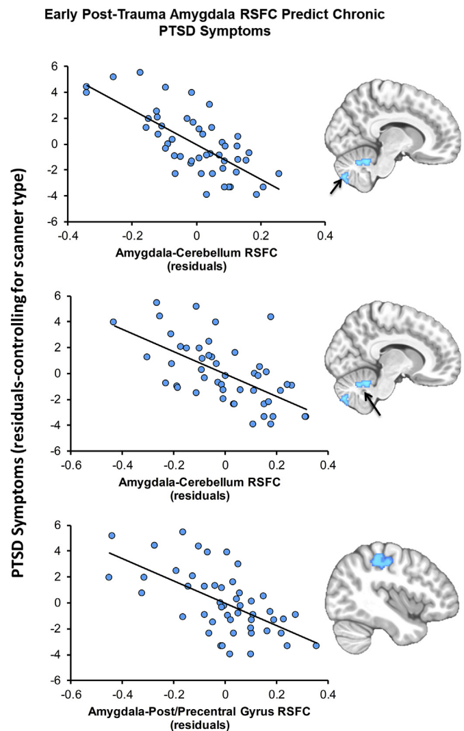
Fig. 1. Early post-trauma amygdala resting state functional connectivity (RSFC) predicted greater six-month post-trauma PTSD symptom severity.
