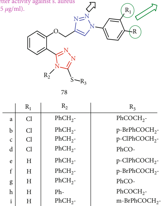
FIGURE 59: Assessment of bis-1,2,4-triazole derivatives as antifungal agents.
