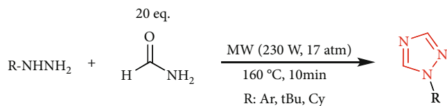
SCHEME 2: The preparation of 1,2,4-triazoles from hydrazines.
