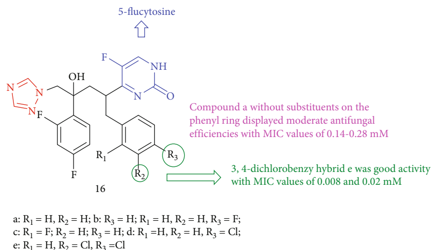
FIGURE 16: Structure of novel t hybrids of 5-flucytosine and fluconazole.
