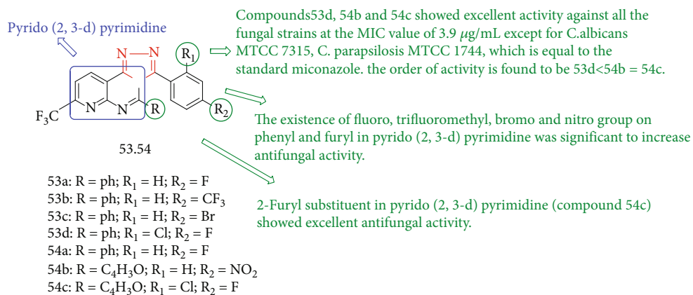
FIGURE 43: Chemical structure of new 4-hydrazono functionalized/1,2,4-triazole fused pyrido [2,3-d] pyrimidine derivatives.
