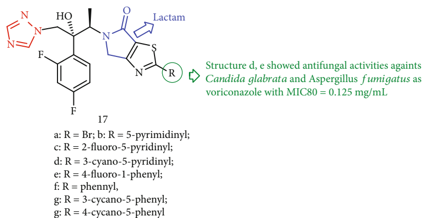
FIGURE 17: Novel triazole derivatives bearing \gamma -lactam.
