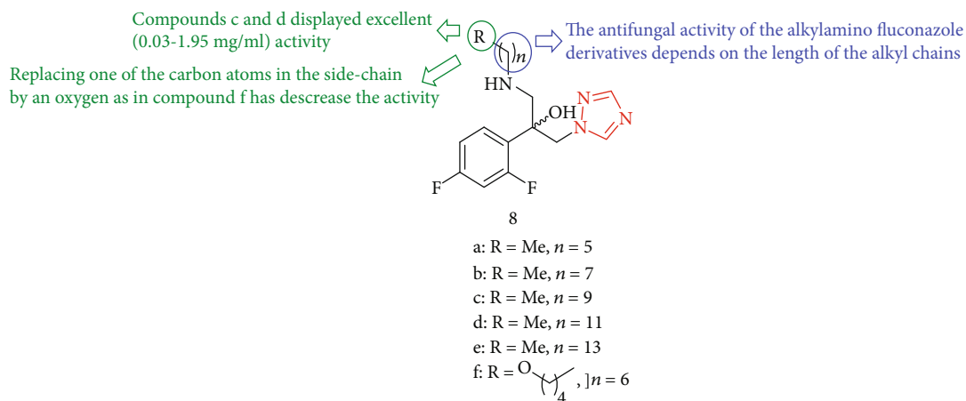
FIGURE 10: The study of antifungal properties in new fluconazole derivatives.
