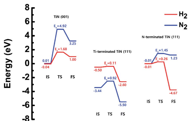
Fig. 4 Calculated energy diagram of H 2 and N 2 decomposition on the TiN (001), the Ti-terminated TiN (111), and N-terminated TiN (111) surface.
