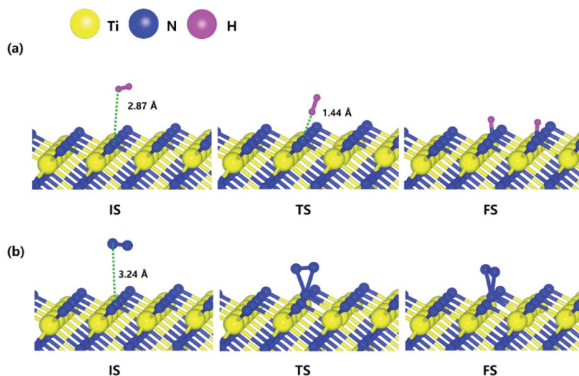
Fig. 3 The optimized initial, transition, and final structures of the dissociative chemisorption step for (a) H 2 and (b) N 2 on the N-terminated TiN (111) surface.
