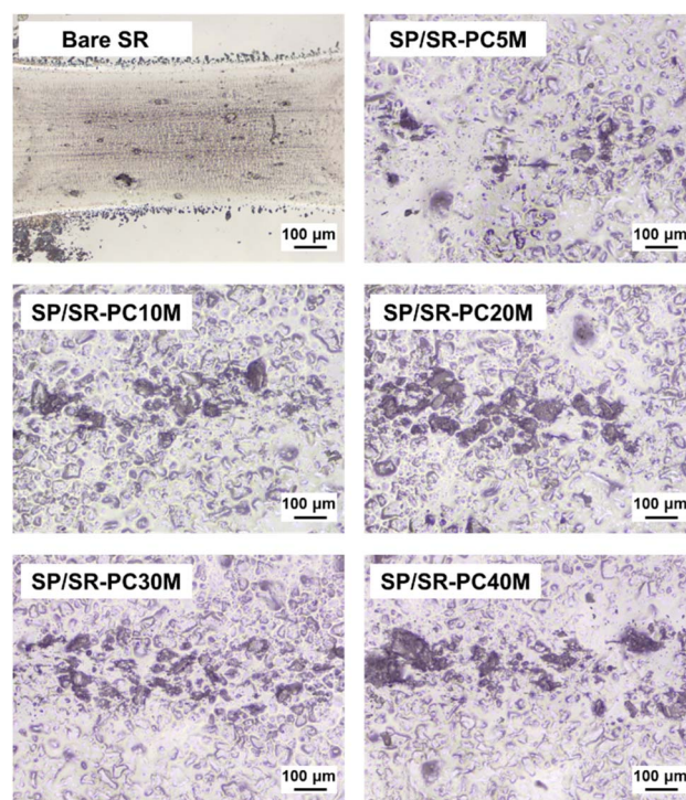
Fig. 6 Optical microscope images of wear tracks formed on the surfaces of bare silicone rubber and silicone powder-coated silicon rubbers according to the pre-curing time.
