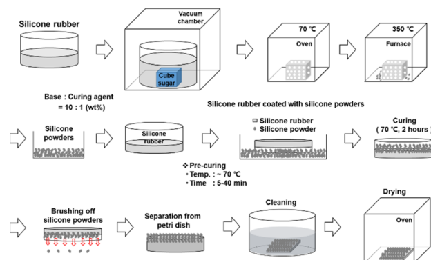
Fig. 1 Fabrication process of silicone powder-coated silicone rubbers.
