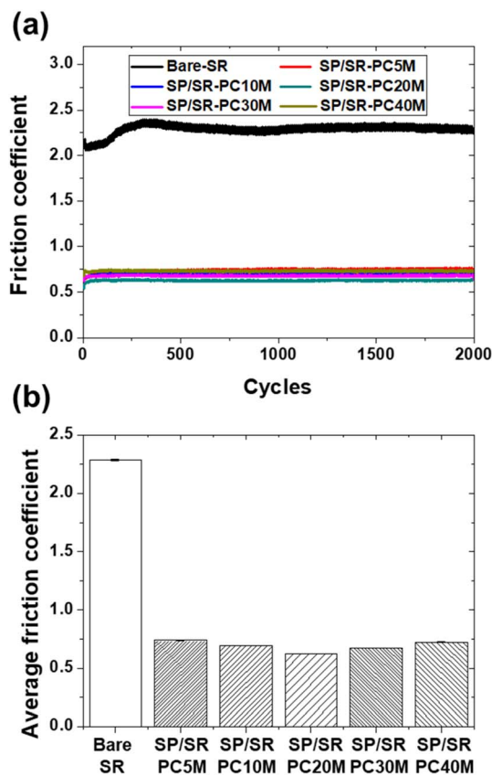
Fig. 5 Friction characteristics of bare silicone rubber and silicone powder-coated silicon rubbers according to the pre-curing time: (a) friction coefficient history and (b) average friction coefficient.
