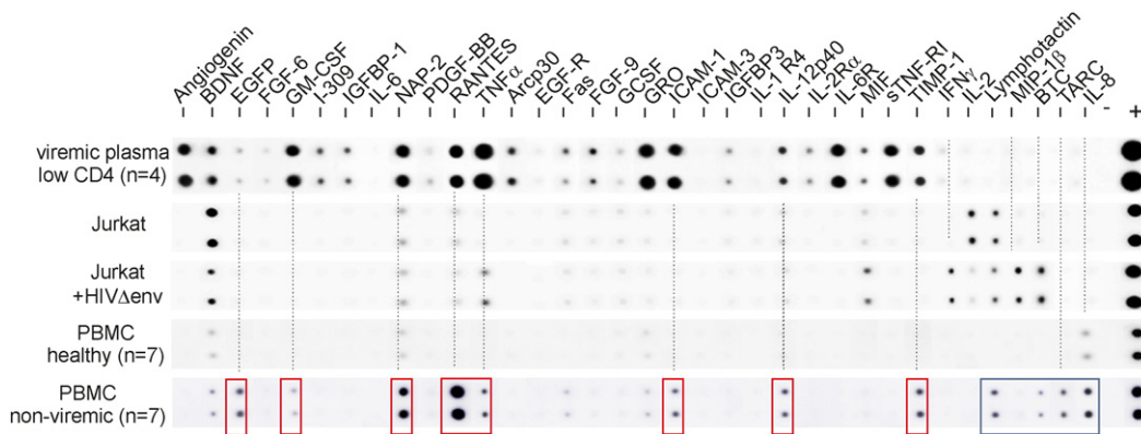
Fig. 7. PBMC-derived CCF contribute to HIV pEV. Protein array analyzing the content of cytokines, chemokines and soluble factors (CCF) in EV purified from culture supernatants of Jurkat T cells transfected with a HIV- \Delta env construct for 72 h or vector control (expression control in Fig. S6B), and from resting PBMC from 7 non-viremic individuals and 7 healthy controls cultured separately for 48 h. For comparison, pEV were purified from plasma pools of viremic/non-viremic patients as described in Fig. 2B. See full CCF list analyzed in supplementary information. Assay input details are summarized in Table S2.
