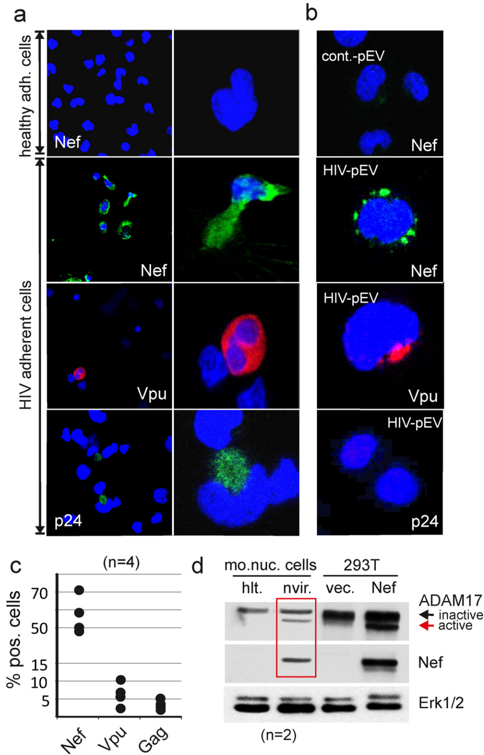
Fig. 4. Peripheral mononuclear cells ingest large amounts of HIV pEV. Immunohistochemistry analysis of Nef, Vpu and p24 Gag in plastic adherent PBMC, obtained from non-viremic patients and a healthy controls. (a) One representative sample is shown. (b) Nef, Vpu and Gag staining as in (a) after incubation of non-viremic HIV pEV (gradient-purified) with plastic-adherent PBMC from a healthy individual. (c) Average number of positive cells (in %) stained as in (a) in 4 non-viremic patients. For each patient 3.0 \times 10^2 cells were analyzed and the mean value was taken as a representative number. (d) Western blot analysis of plastic adherent cells from one non-viremic individual (nvir.) and one healthy control (hlt.) for factors as indicated. Nef/co-factors-transfected cells 293 T cells (as in Fig. 3a) served as positive control.
