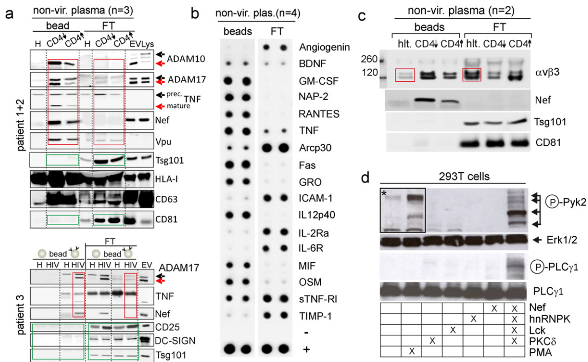
Fig. 3. HIV pEV constitute a pEV subclass induced by \alpha v \beta 3 activation. (a) HIV pEV isolation from plasma of 3 non-viremic patients with high or low CD4 count using 2H4-coupled magnetic beads (see Fig. S2). Bead isolated pEV (bead) and flow through (FT) were analyzed for the indicated markers. The lower panel includes an additional control for non-coupled beads, indicated by a sphere w/o antibody. Red and green boxes point to differences between bead-isolation and FT (details in text). (b) CCF protein array analysis of purified pEV from non-viremic patients (30 ml pooled plasma, 4 patients) coupled to 2H4-coupled beads (beads) and flow through (FT). (c) Same experimental set up as in (a). pEV were isolated from two non-viremic patients using 2H4-coupled beads and blotted for indicated markers. Red boxes refer to differences in bead-isolated fraction and flow through as described in the text. (d) Expression of Nef and co-factors in 293 T cells as indicated and similar as performed previously (Lee et al., 2013), and immunoblot for phosphorylated endogenous Pyk2 and PLC \gamma . Insert*: longer exposure of negative control and PMA stimulation as compared to the rest of the blot.
