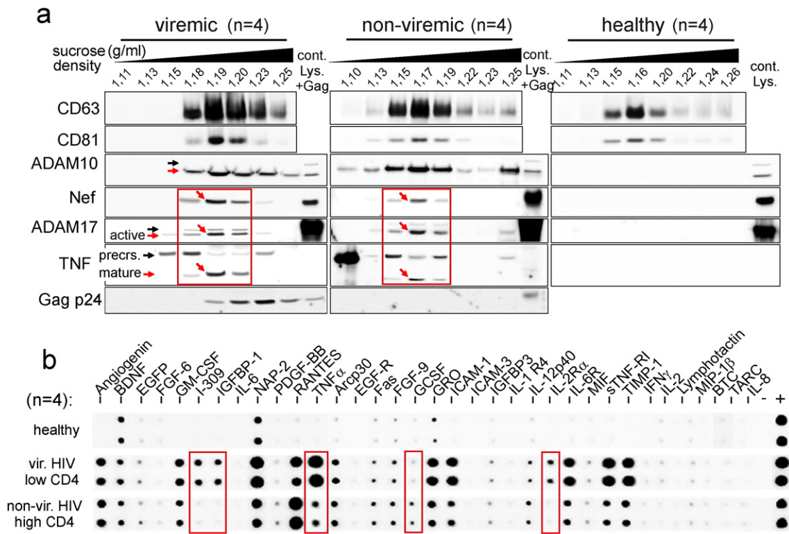
Fig. 2. HIV pEV contains viral accessory proteins and inflammatory effectors. (a) Western blot analysis of individual sucrose gradient fractions from viremic and non-viremic patients. Purified pEV from samples analyzed in Fig. 1d and viremic patients (n = 4, pools of 24 ml each) were blotted for indicated factors. Red arrows in the boxes depict the positive correlation of Nef with ADAM17 and pro-TNF cleavage, precurs.: precursor. Note: CD63 and CD81 western blot panel in Fig. 1d and panel (a) in this figure are identical (same samples). Lysates of 293 T cells, transfected with p24 Gag (+ Gag) and/or Nef/Nef-cofactors (Lys.), served as controls (Cont.). (b) Protein array analyzing the content of cytokines, chemokines and soluble factors (CCF) in pEV from healthy controls, viremic patients with low CD4 counts (120–250/μl) and non-viremic HIV patients with high CD4 counts (>750/μl) (30 ml pooled plasma, 5 patients). See full CCF list analyzed in supplementary information.
