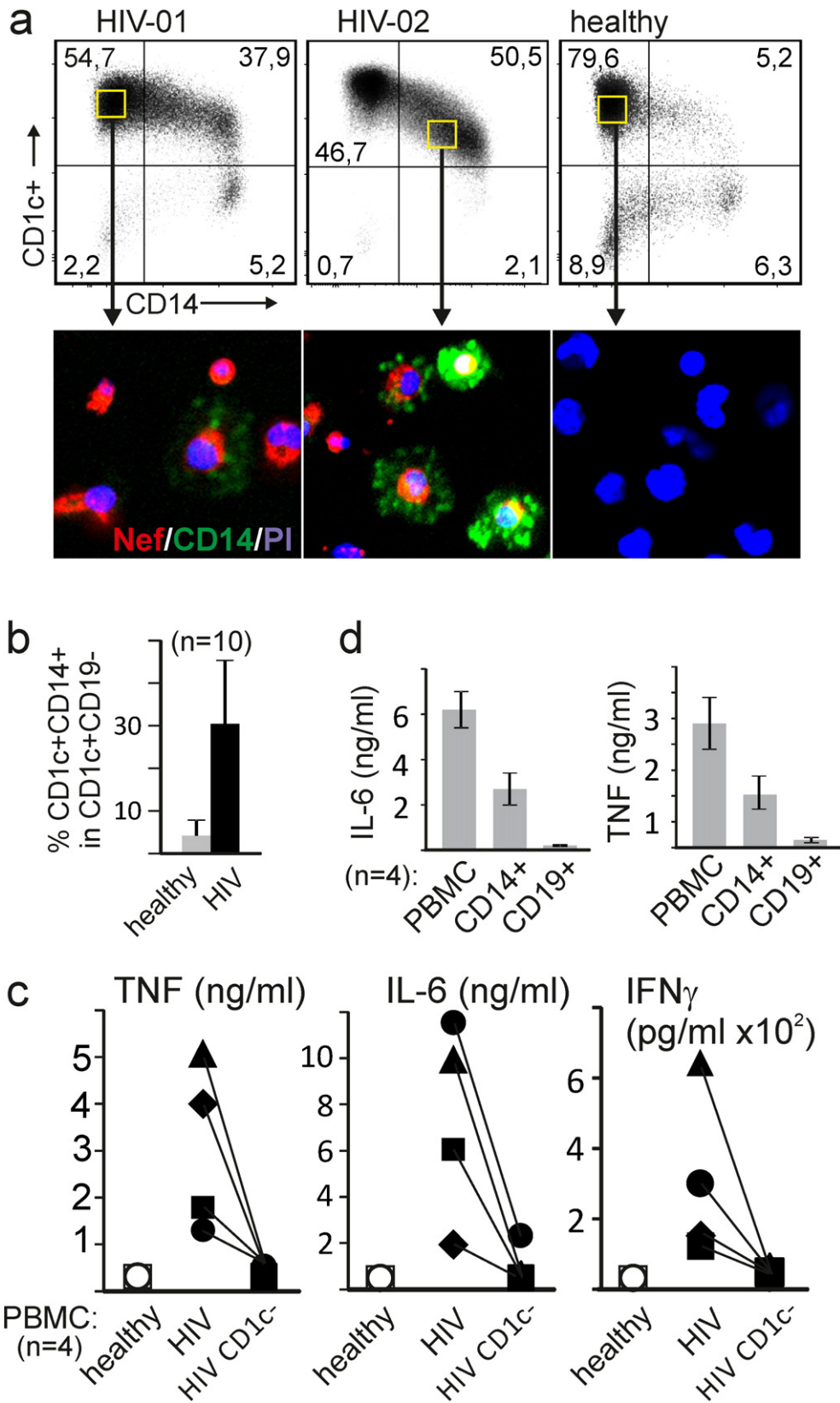
Fig. 5. CD1c + CD14 + mononuclear cells contain Nef and secrete inflammatory cytokines. FACS and immunohistochemistry analysis of Nef-containing mononuclear cells. (a) Assessment of CD1c + CD14 + cells in CD1c + positive selected PBMC from 2 non-viremic patients and a healthy control. Aliquots of the cells were stained for Nef and CD14 by immunohistochemistry. (b) Percentage of CD1c + CD14 + cells in the CD1c + CD19 - cell fraction based on the analysis of 5 non-viremic patients and healthy controls. Error bars represent mean \pm SEM. (c) Secretion of TNF, IL-6 and IFN \gamma by 10 5 PBMC obtained from 4 non-viremic patients and controls in 12 h. PBMC were left untreated or the CD1c + fraction was positive depleted (by magnetic beads) (d) TNF and IL-6 secretion from PBMC, or from 10 5 positive-selected CD14 + and CD19 + cells in 12 h. Error bars show the SEM.
