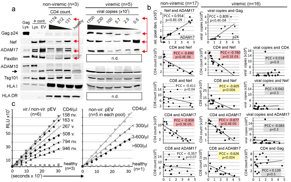
Fig. 6. pEV-derived Nef and ADAM17 activity correlate with low T cell counts. (a) Correlation of pEV protein levels of Nef and other markers with CD4 count (left panel, arrows) and viral copy numbers (right panel, arrows). Plasma-EV were purified by differential centrifugation from non-viremic and viremic patients. The equivalent of 3 ml plasma was analyzed by Western blot. Lysates (Lys.) of 293 T cells, transfected with p24 Gag (Gag Lys.) or Nef/Nef-cofactors (+ cont.), served as controls, as well as EV purified from these transfected cells (EV). (b) Correlation and significance analyses (Pearsons correlation coefficient (PCC); Student's t-test) of pEV-derived Nef-, ADAM17- and p24 Gag-levels with CD4-, CD8-count and viral copy numbers. Protein-levels were assessed from 16 viremic and 17 non-viremic patients (see Figs. S3 and S4) by Western blot and quantified by ImageJ. Boxes were colored to simplify their explanation in the text. (c) Correlation of ADAM17 activity with CD4 count. Plasma EV were purified from 6 viremic and non-viremic patients and 3 healthy controls (left panel), and from 30 ml of pooled plasma (5 patients, 6 ml each), collected from non-viremic HIV patients with different CD4 counts as depicted. Aliquots corresponding to 1 ml of plasma were analyzed using a commercial assay (AnaSpec).
