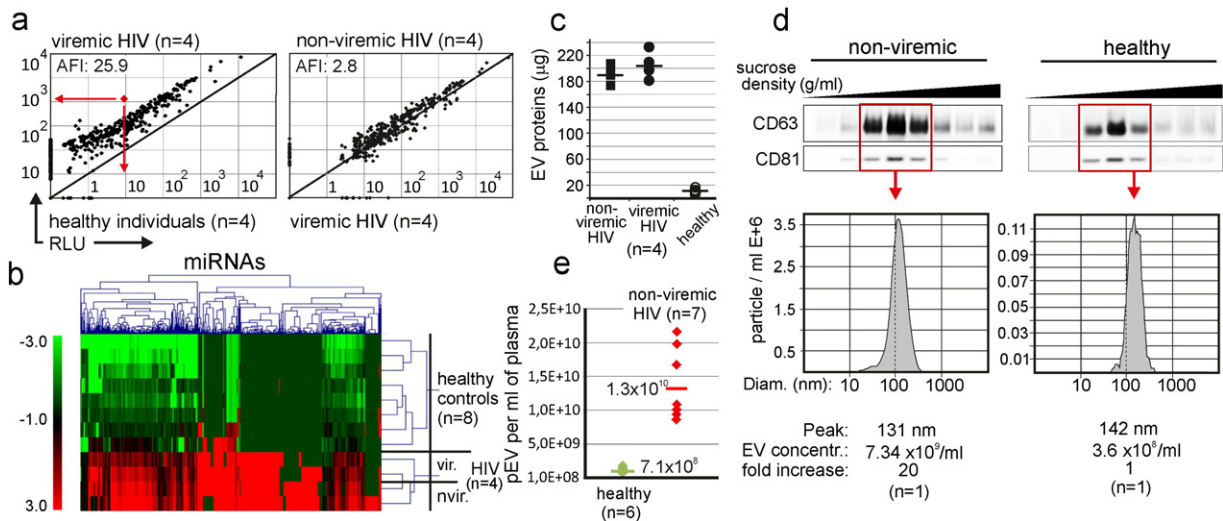
Fig. 1. High levels of Nef-containing pEV in viremic and non-viremic HIV infection. (a) Pairwise comparison of pEV miRNA levels obtained by miRNA micro arrays, derived from viremic HIV patients and healthy controls (left panel), and non-viremic patients (right panel). Each dot depicts the signal intensity of one miRNA, exemplified by the red dot and arrows. The pEV were extracted by sucrose gradient from 24 ml of pooled plasma (4 individuals, 6 ml each). AFI: average fold-increase of all miRNAs over reference. RLU: relative light units. (b) Hierarchical clustering based on Euclidean distance of miRNAs extracted from pEV (14 ml plasma) from 8 healthy individuals and 2 viremic ( 2.1 \times 10^4 and 5.6 \times 10^3 viral copies/ml) and 2 non-viremic HIV-infected individuals. nvir.: non-viremic. vir.: viremic. (c) Protein levels (µg) in sucrose gradient fractions 1.13–1.23 (as in Fig. 1D) from viremic ( 10^3 – 10^5 viral copy numbers/ml) and non-viremic patients (<20 viral copies/ml) as well as controls (n = 4). (d–e) Particle number and size analysis of pEV. (d) Example of a pEV analysis from a pool of non-viremic individuals and healthy controls (n = 4, pools of 24 ml each), subjected to a concentration analysis by dynamic light scattering using a ZetaView® nanoparticle tracker (ParticleMetrix GmbH; Meerbusch, Germany). (e) Gradient-purified pEV derived from 15 ml plasma from 7 non-viremic individuals and 6 healthy controls using the ZetaView® nanoparticle tracker. Based on the measurements a pEV concentration per ml plasma was calculated as indicated.
