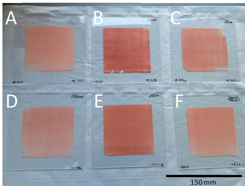
Fig. 7 Catalyst plates with a 150 × 150 mm size and a coated area of 100 × 100 mm each. A = 1–2 nm, B = 50 nm, C = 100 nm, D = 200 nm plate, A, E = 200 nm plate and B, F = 370 nm porous glass.
