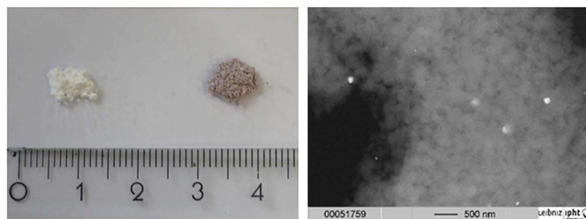
Fig. 1 Left: Photo of samples ground with no metal salt (white powder), and with \text{HAuCl}_4 (purple powder). Right: The SEM images of the samples with \text{HAuCl}_4 /glass after grinding show a few gold nanoparticles in the bulk (bright structures).
