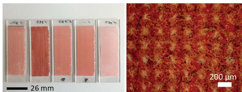
Fig. 2 Gold particles laser sintered on the object slides (left image; from left to right: \text{HAuCl}_4 with 1–2, 50, 100, 200 and 370 nm porous glass). A light microscopy close up view with 5\times magnification of the coating structure with gold nanoparticles (right image). Here, the course of the laser is visible in the red sintered grids with particles and the white non-sintered spaces containing no particles.
