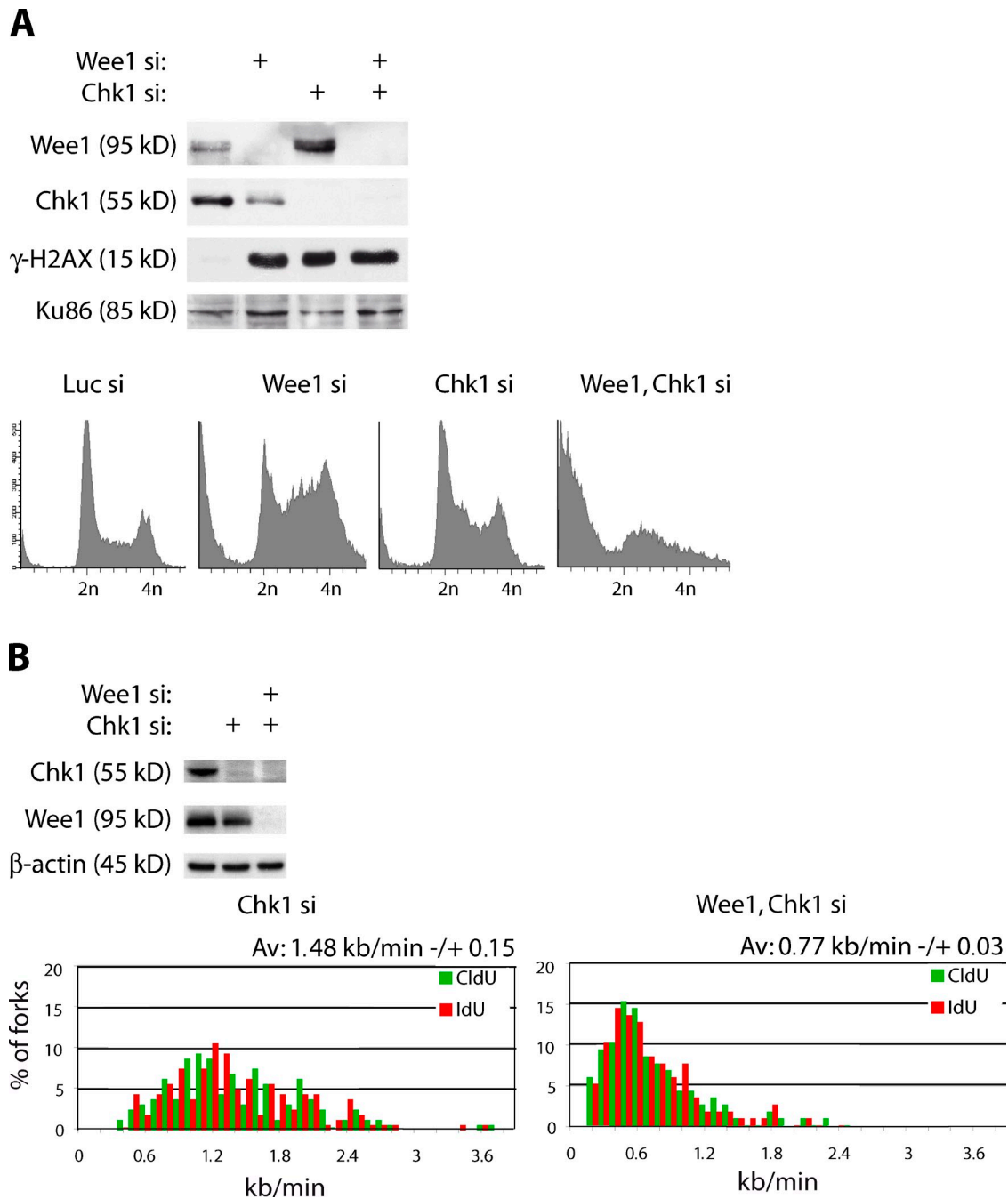
Figure 5. Wee1 and Chk1 protect from replication problems in a different manner. (A) Flow cytometry analysis after propidium iodide staining (bottom) and immunoblot analysis (top) of U2OS cells transfected with Luc, Wee1, or Chk1 siRNA oligonucleotides or a combination for 48 h. (B) U2OS cells were transfected with Chk1 with or without Wee1 siRNA oligonucleotides for 48 h and thereafter pulsed for IdU and CldU. (bottom) Fork speed was determined by measuring the length of IdU and CldU tracks on combed DNA molecules. Bar graphs show the percentages of molecules with certain replication speeds from one representative experiment. Above each graph, the mean fork speed with the SEM of three independent experiments is indicated. (top) Levels of the indicated proteins by Western blotting.
