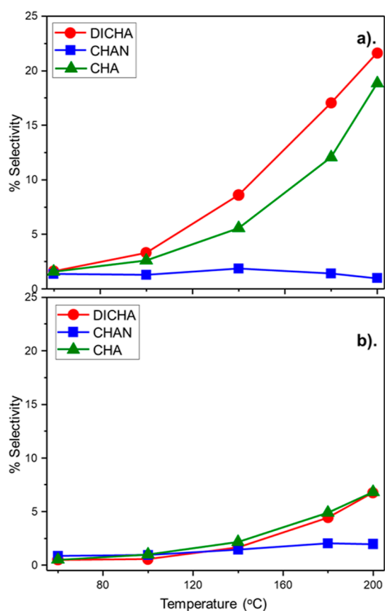
Figure 5. ANL overhydrogenation by-products DICHA, CHAN, and CHA as a function of temperature in the presence of an enhanced flow of dihydrogen: ( \text{H}_2/\text{C}_6\text{H}_5\text{NO}_2 molar flow ratio = 600:1 and \text{WHSV} = 0.20 \text{ h}^{-1} ): (a) GU-3 and (b) GU-4.
