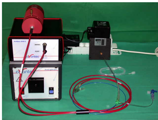
Figure 1 NIR spectroscopy: The fiberoptic catheter is connected to the spectrophotometer and the halogen light source (red).
