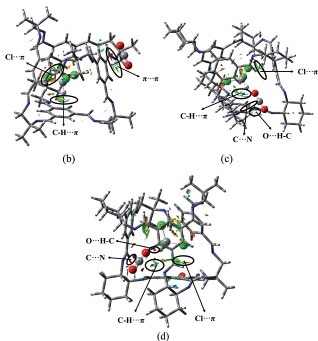
Fig. 8 (a) Plots of the electron density and its reduced density gradient (SYS-e). Gradient isosurfaces ( s = 0.35 a.u.) for (b) COM-f. (c) ABS-e. (d) SYS-e. The surfaces are colored on a red-green-blue scale according to values of \sin(\lambda_2)\rho , ranging from -0.01 to 0.02 a.u. Red indicates strong attractive interactions, and blue indicates strong nonbonded overlap.
