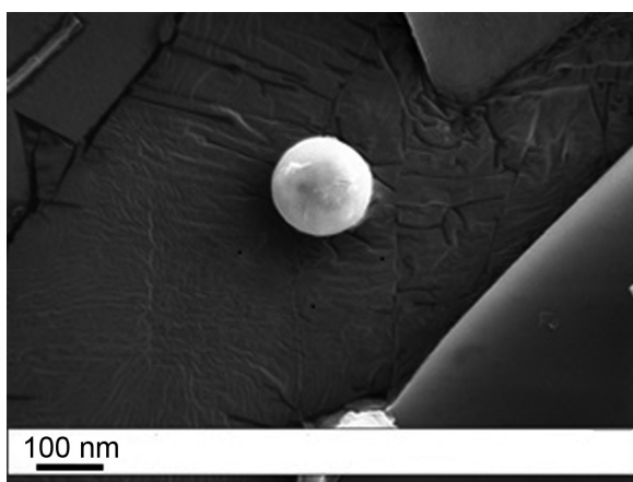
Figure 1 SEM image of optimized FLV-NLCs. Abbreviations: SEM, scanning electron microscope; FLV-NLCs, fluvastatin nanostructured lipid carriers.
