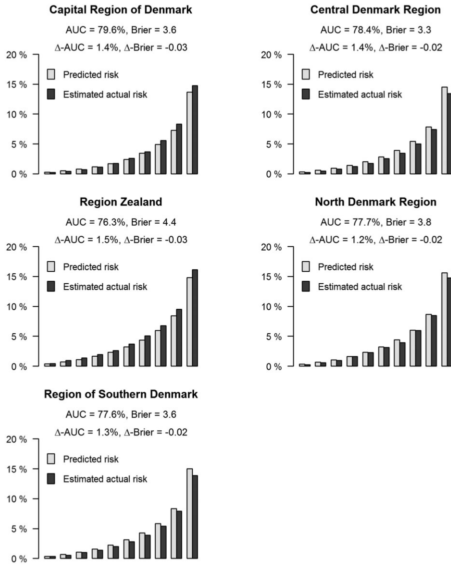
Figure 4 Calibration plots and discrimination metrics across the five regions. The predicted risk is plotted in deciles against the estimated actual risk. Differences in AUC and Brier scores compared to an age-sex benchmark model is presented as delta-AUC and delta-Brier. AUC, area under the receiver operating characteristic curve.
