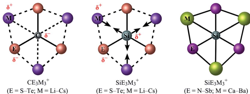
Fig. 1 The pictorial depiction of previously reported phC CE_3M_3^+ (E = S–Te; M = Li–Cs) clusters and the present SiE_3M_3^+ (E = S–Te and N–Sb; M = Li–Cs and Ca–Ba) clusters. Herein the solid and dashed lines represent covalent and ionic bonding, respectively. The opposite double arrows illustrate electrostatic repulsion.
