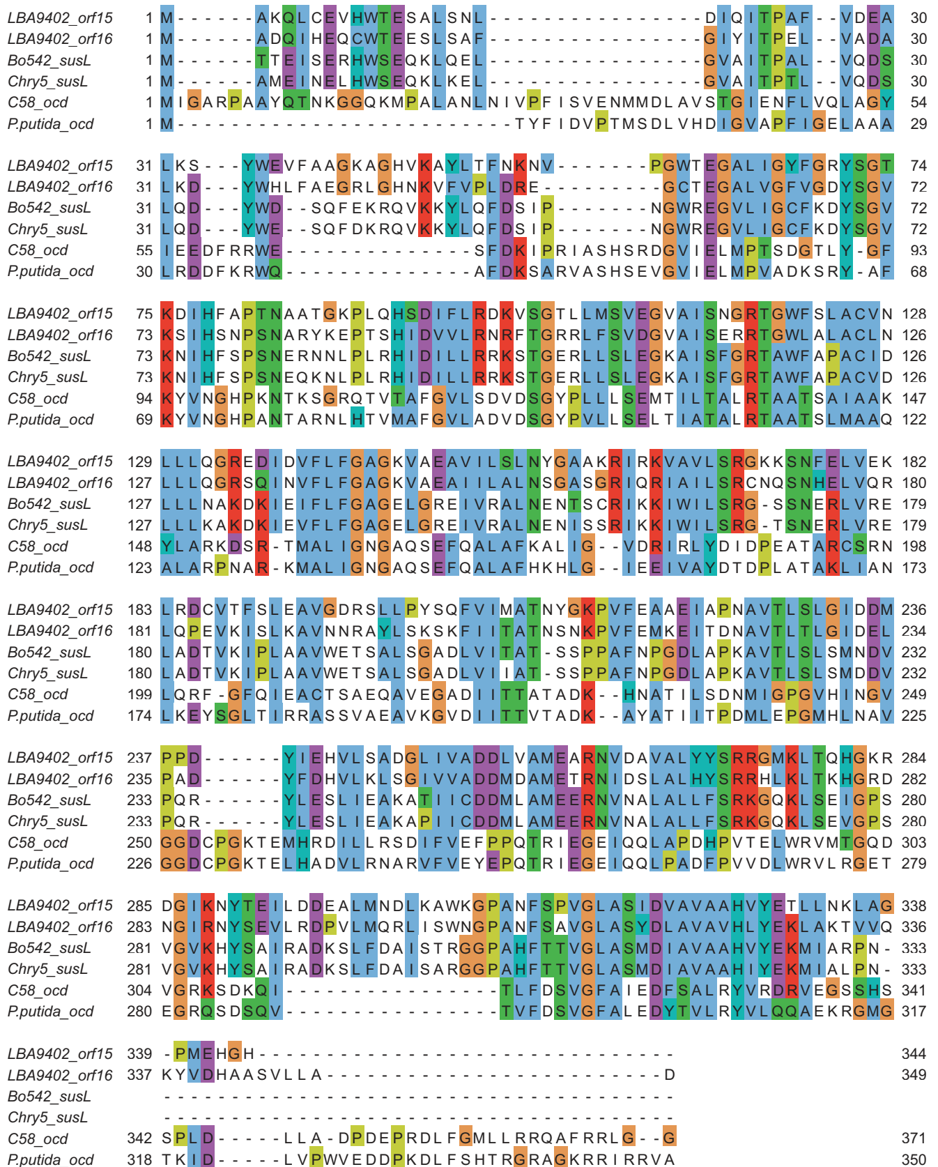
FIGURE 4 The proteins encoded by orf15 and orf16 are evolutionarily related to succinamopine synthase and more distantly to ornithine cyclodeaminase. Multiple sequence alignment of proteins encoded by orf15 and orf16 of pRi1855, susL from A. tumefaciens strains Chry5 and Bo542, and ocd from A. tumefaciens C58 and Pseudomonas putida . Colors are according to the Clustal X color scheme
