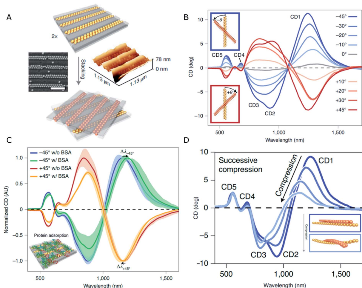
Fig. 2 (A) Schematics of the stacking method, and SEM and AFM characterization of dimer chains formed from Au NPs assembled on 1D patterned templates (scale bar is 500 nm). (B–D) CD spectra obtained for different stacking angles (B), in the presence of BSA (C), and upon compression applied normal to the stacking plane (D). Adapted from ref. 79 with permission from Nature Publishing Group, copyright 2021.
