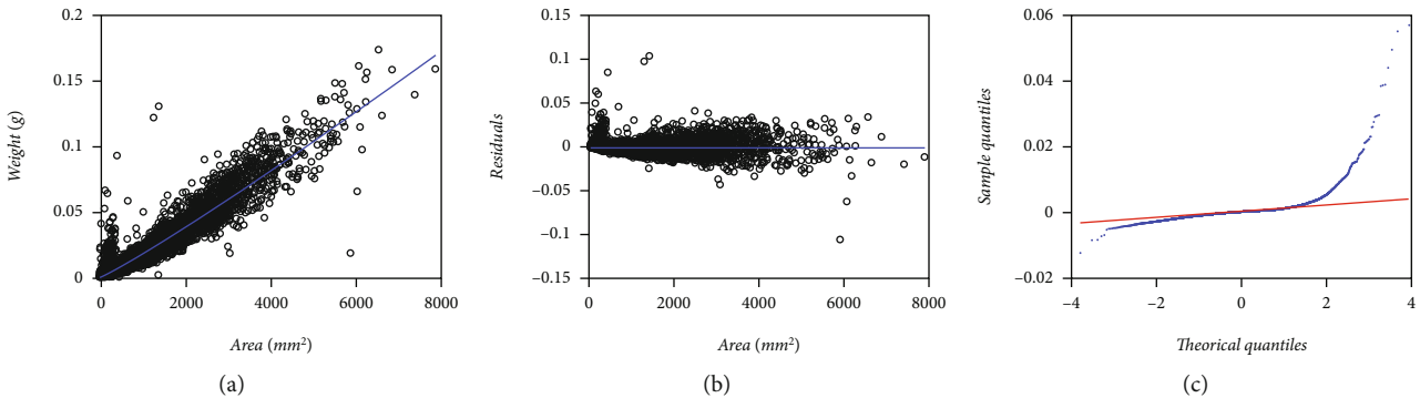
FIGURE 5: Spreads about mean response curve, that of residual and the one portraying in the Q-Q normal plot of the heteroscedastic DNLB-BP scheme of Equations (10) and (12) fitted on the Echavarría-Heras et al. [37] data set. (a) Dispersion about fitted Huxley’s power function form. (b) The scatter diagram of residuals against leaf area. (c) The Q-Q normal plot of the residuals on direct arithmetical scales. Heavy tails appear through a markedly asymmetrical pattern which refers to an overall inconsistent DNLB-BP fit.
