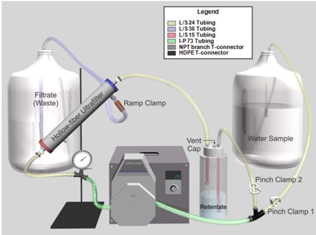
Figure 1. Graphic representation of the tangential flow hollow-fiber ultrafiltration system. The tubing is color coded to aid in assembly of the system.
