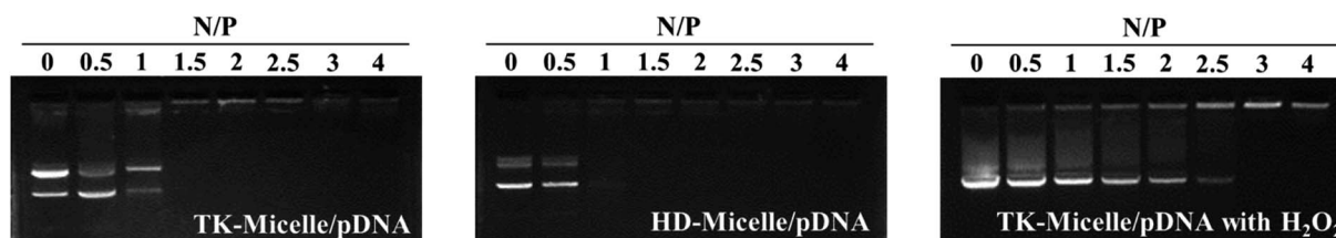
Fig. 2 The agarose gel electrophoresis of the TK-Micelle/pDNA, HD-Micelle/pDNA, and TK-Micelle/pDNA with H 2 O 2 (50 \mu\text{M} ) at various N/P ratios.
