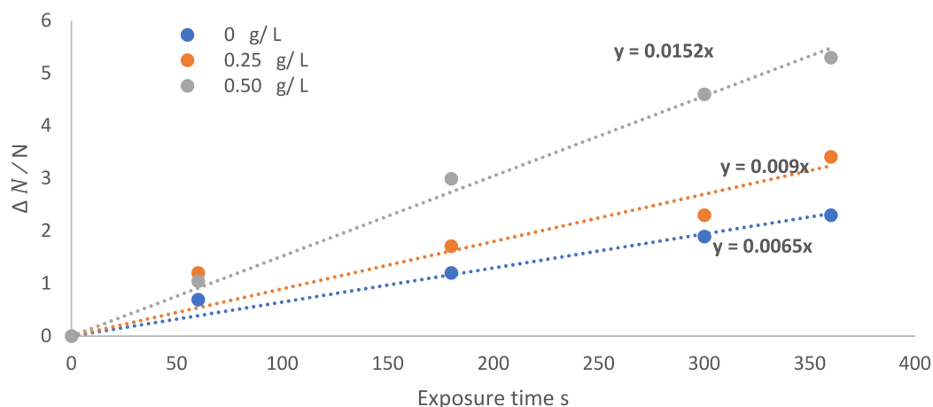
Figure 8. \Delta N/N_0 as a function of exposure time at different \text{TiO}_2 concentrations, 0, 0.25, and 0.50 g/L, coupled with dry argon APPJ discharge.
