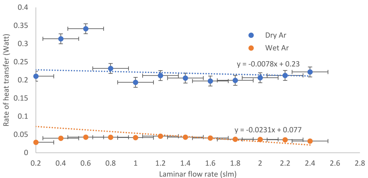
Figure 3. Heat impacting the bacterial colonies as a function of laminar mode flow for dry and wet argon discharge.
