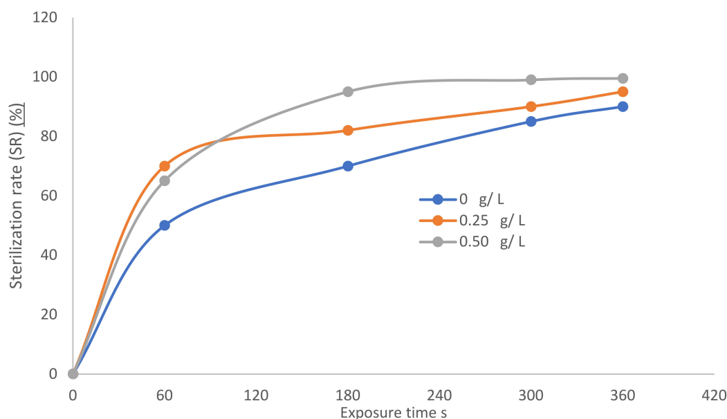
Figure 9. Sterilization rate (SR) (%) versus exposure time.
