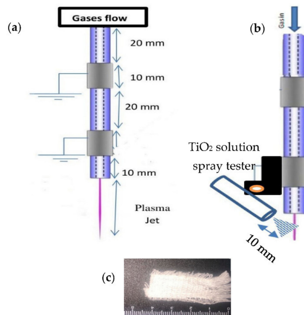
Figure 1. (a) Experimental setup of dry Ar-APPJ discharge, (b) wet Ar-APPJ discharge, and (c) the woven cotton fabric control (untreated sample).
