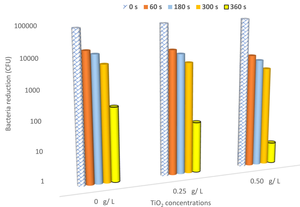
Figure 7. Bacterial reduction (logarithmic scale) in the cell-forming unit per milliliter (CFU/mL) as a function of \text{TiO}_2 concentration: 0, 0.25, and 0.50 g/L.
