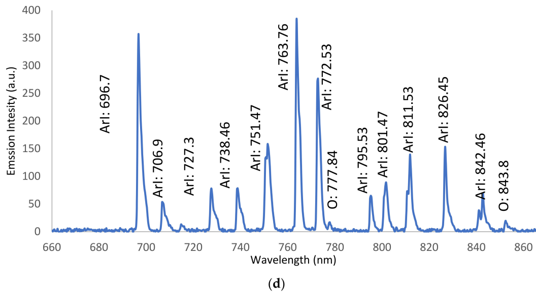
Figure 4. (a). Intensity of emission spectra versus wavelength for dry argon discharge. (b) Intensity of emission spectra versus wavelength for the hydroxide band. (c) Intensity of emission spectra versus wavelength for nitrogen bands. (d) Intensity of emission spectra versus wavelength for argon with oxygen line.
