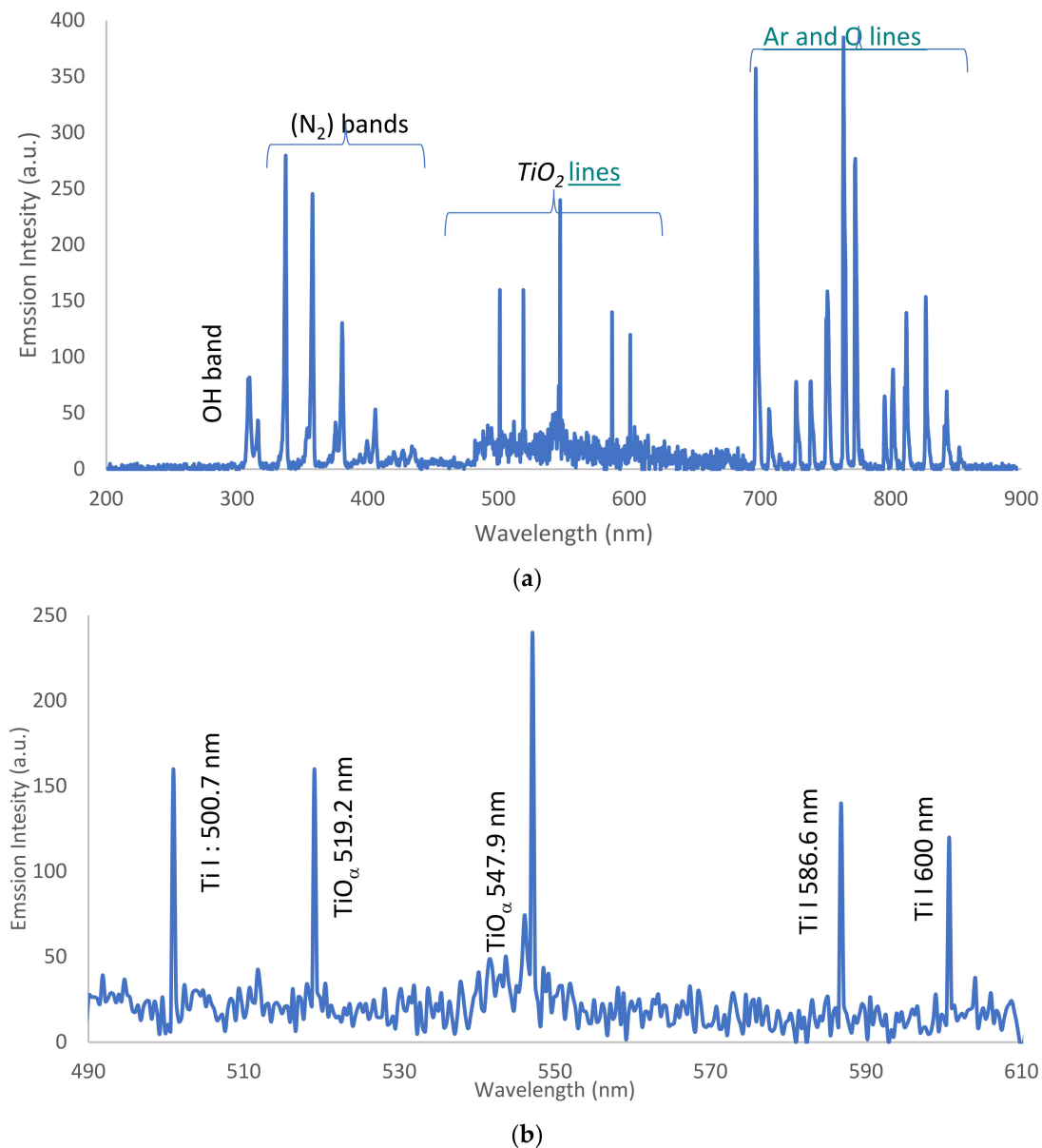
Figure 5. (a) Intensity of emission spectra versus wavelength for wet argon discharge. (b) Intensity of emission spectra versus wavelength for TiO 2 lines.
