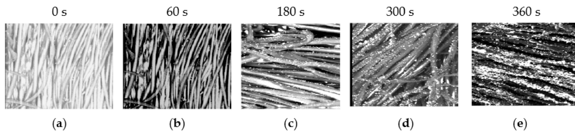
Figure 6. SEM micrographs of the cotton fabric samples before and after APPJ sputtering treatment: (a) controlled sample without treatment, (b) sample treated with dry Ar-APPJ for an exposure time of 60 s; (c–e) samples treated with wet Ar-APPJ for an exposure time of 180, 300, and 360 s, respectively.
