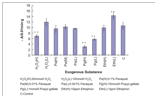
Figure 2: Effect of H_2O_2 , paraquat, propyl gallate, and ethephon on peroxidase activity. Groups of data were compared with an analysis of variance followed by multiple comparison tests. * P < 0.05 versus control group; ** P < 0.01 versus control group
