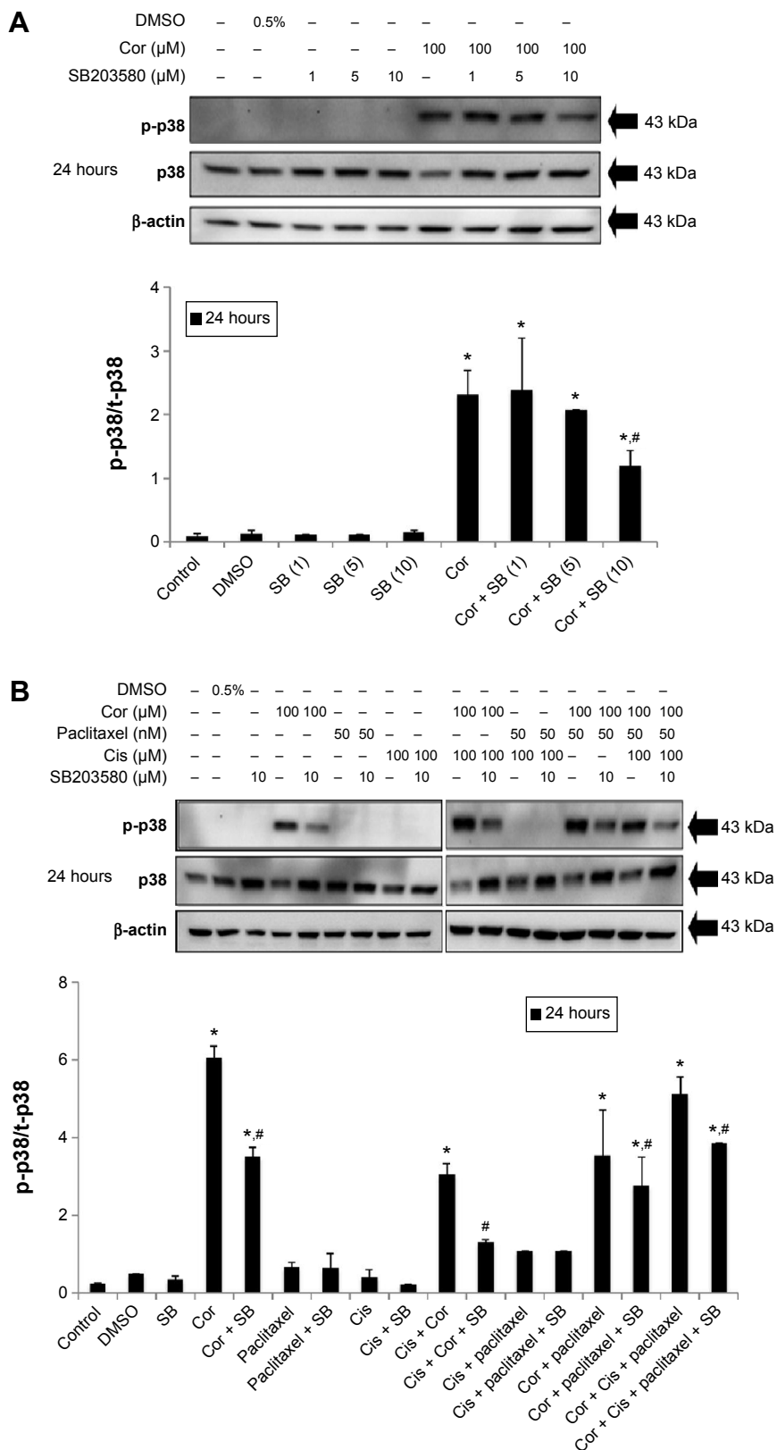
Figure 7 The p38 inhibitor (SB203580) reversed cordycepin- + paclitaxel- and/or cisplatin-induced phosphorylation of p38 in MA-10 cells. Notes: The cells were pretreated with 1, 5 and 10 \mu\text{M} SB203580 (SB) for 30 minutes, and then cotreated without or with 100 \mu\text{M} cordycepin and 1, 5, and 10 \mu\text{M} SB203580 for 24 hours (A), or without or with 50 nM paclitaxel and/or 100 \mu\text{M} cisplatin +100 \mu\text{M} cordycepin and 10 \mu\text{M} SB203580 for 24 hours (B). After 24 hours, t-p38 (43 kDa) and p-p38 (43 kDa) were detected by Western blots. The integrated optical density of p-p38 protein expression after normalization with t-p38 is demonstrated. Each datum point in the figure represents the mean \pm standard error of the mean of three separate experiments. *Indicates a statistically significant difference compared with control ( P < 0.05 ). #Indicates that the means are significantly ( P < 0.05 ) different compared with treatments. Abbreviations: p-, phosphorylated; t-, total; Cor, cordycepin; Cis, cisplatin; DMSO, dimethyl sulfoxide; SB, SB203580.
