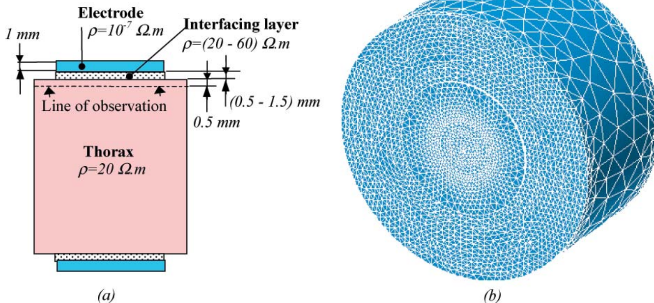
Figure 1 Model of electrode-tissue contact. (a) Disposition of the electrodes (cross-section). (b) Finite-element model with over 50,000 elements.
