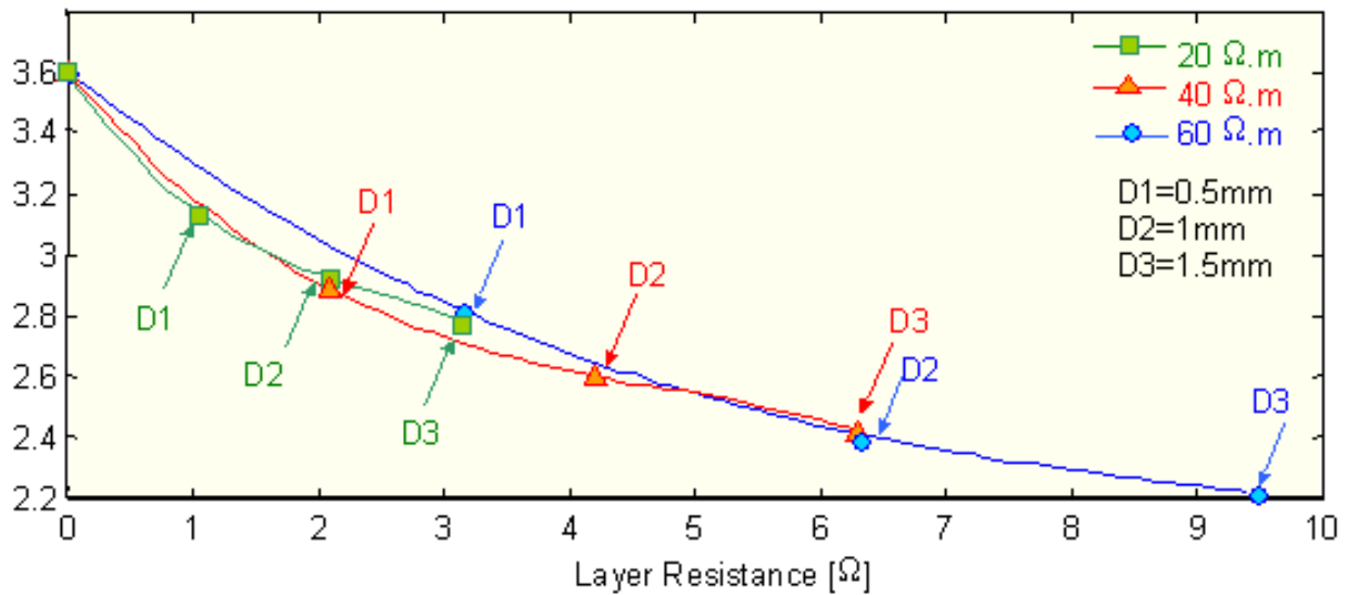
Figure 5 Effect of current density non-uniformity coefficient K of resistance layers with different thickness (D1 = 0.5 mm, D2 = 1.0 mm, D3 = 1.5 mm) and specific resistivity ( \rho = 20, 40, 60 \Omega m ).
