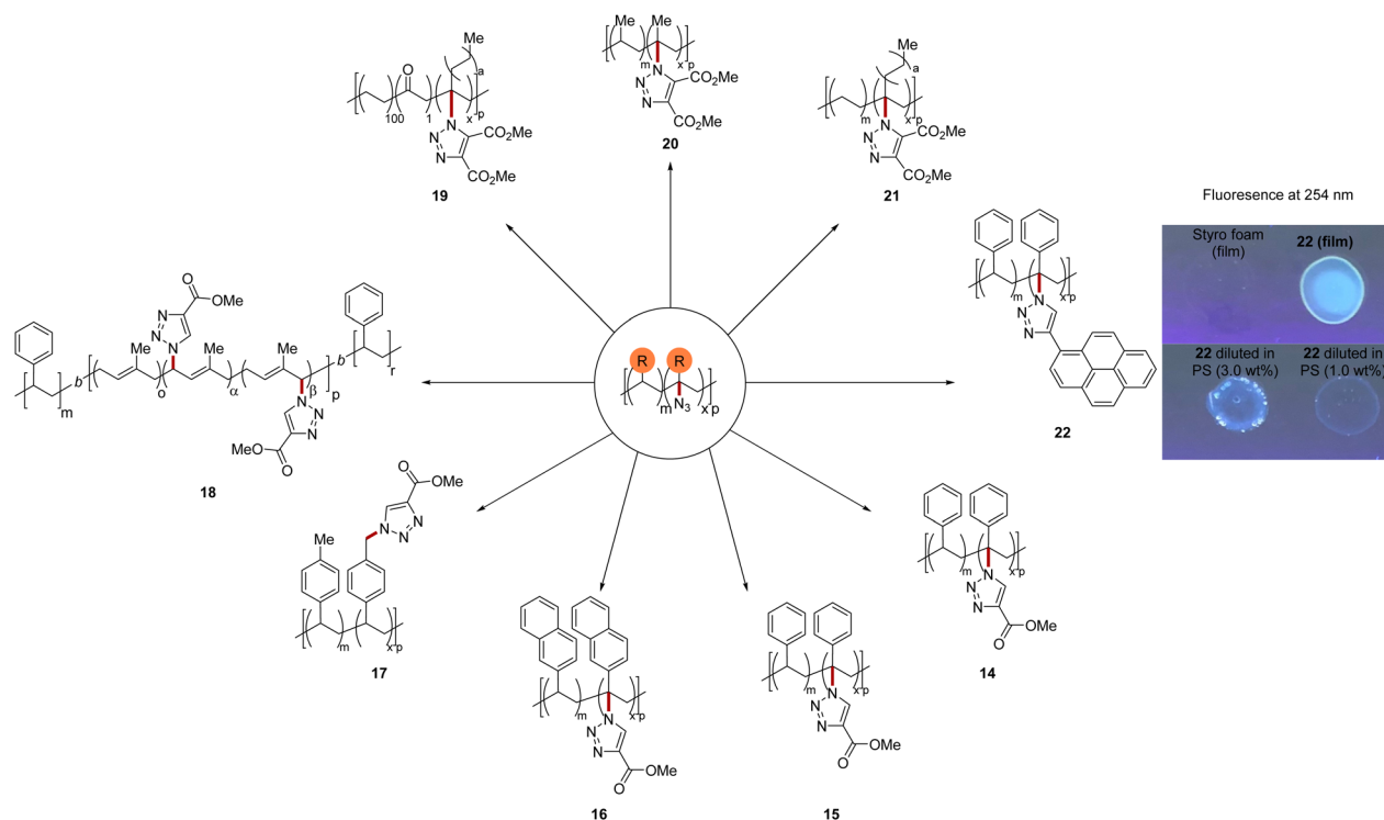
Fig. 5 Product derivatization and fluorescence study. See ESI† for details.
