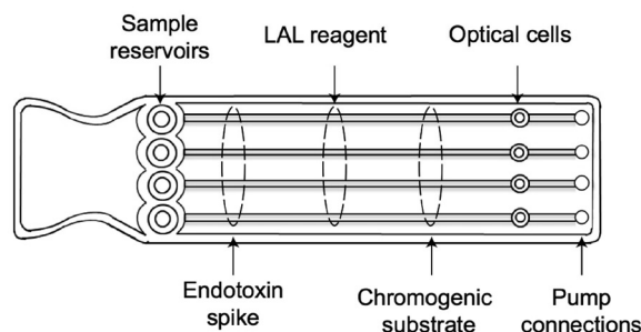
Fig. 1. The Endosafe ® PTS ™ . The limulus amoebocyte lysate (LAL) spectrophotometer (upper) and reagent cartridge (bottom) for PTS ™ .
