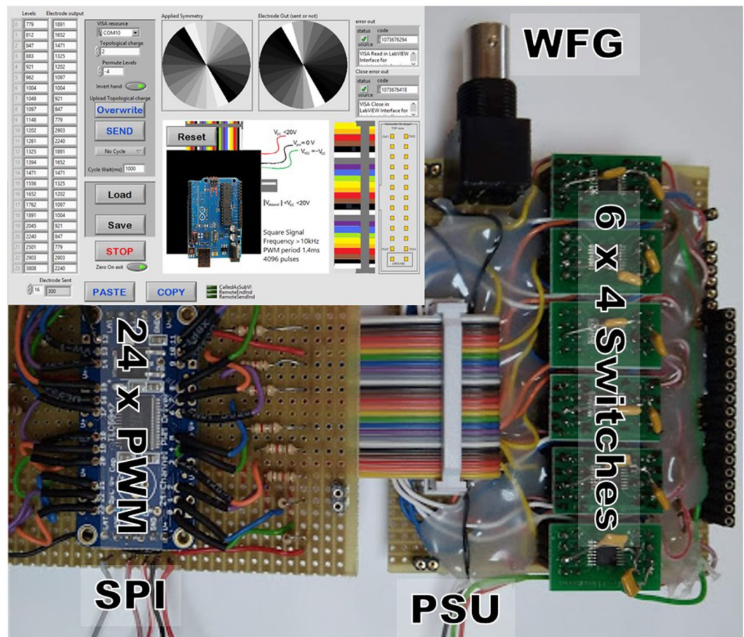
Figure 5. The basic components of the device driver. An array of 24 \times 12 bits is sent to the 24 PWM via the SPI interface. Each of the PWM signals is pulled up by 1.8\text{ k}\Omega resistor to make the output signal transistor-logic (TTL) compatible. Six four channel ADG5412 switches convert the TTL-PWM signals to effective rms voltages (0 to 6 V) for each of the 24 LC signals, by connecting to the 6 V, 10 kHz signal supplied by the waveform generator (WFG). The individual LC electrode is connected to the LC signals, and a 10\text{ k}\Omega pull down resistor. The user interface is included in the insert.
