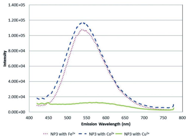
Fig. 9 PL spectra of NP3 in \text{CHCl}_3/\text{CH}_3\text{CN} with 500 nM ( \sim 1 \text{ ppm} ) of \text{Fe}^{2+} , \text{Co}^{2+} and \text{Cu}^{2+} metal ions [reprinted with permission from ref. 89 American Chemical Society].
