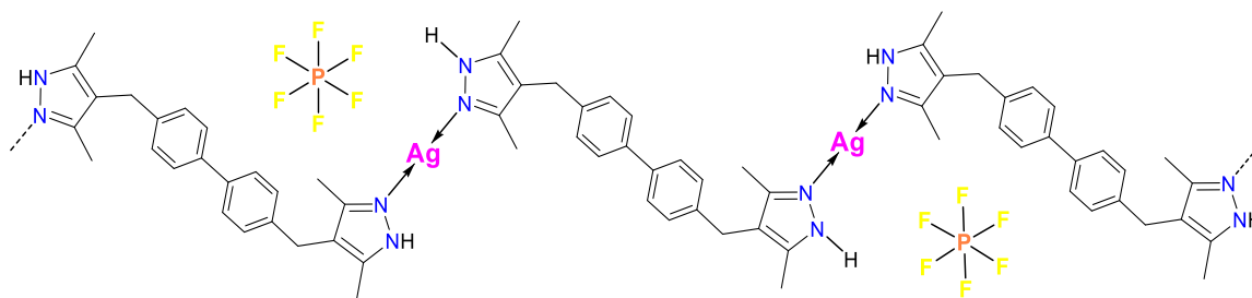
Figure 9. Proposed polymeric structure of [Ag(H_2DMPMB)(PF_6)] ( 6 ), evidencing the digonal stereochemistry of silver(I) ions assured by the neutral ligands coordinated in a bridging exo-bidentate mode.
