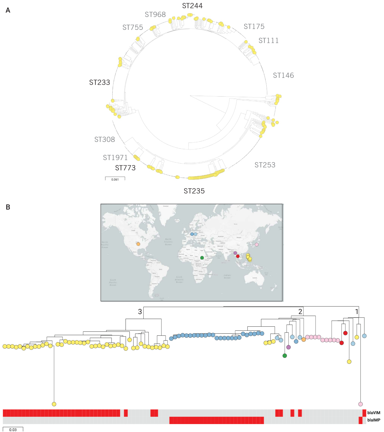
Fig. 3A. Phylogenetic tree of 904 P. aeruginosa isolates from the Philippines ( n = 176 , this study) and from 57 other countries inferred from 549 126 SNP positions. The yellow tree nodes indicate the genomes from this study. The major lineages (STs) are labelled in black if represented by genomes of this study, or in brown if they are not. The data are available at https://microreact.org/project/ARSP_PAE_GLOBAL .
