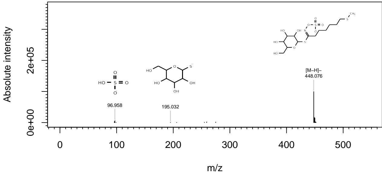
Figure A4. Challenge 4: annotated merged MS/MS spectra of escholtzine (ESI, positive mode).
