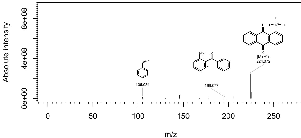
Figure A8. Challenge 11: annotated merged MS and MS/MS spectra of 1-pyrenemethanol (APCI, positive mode).
