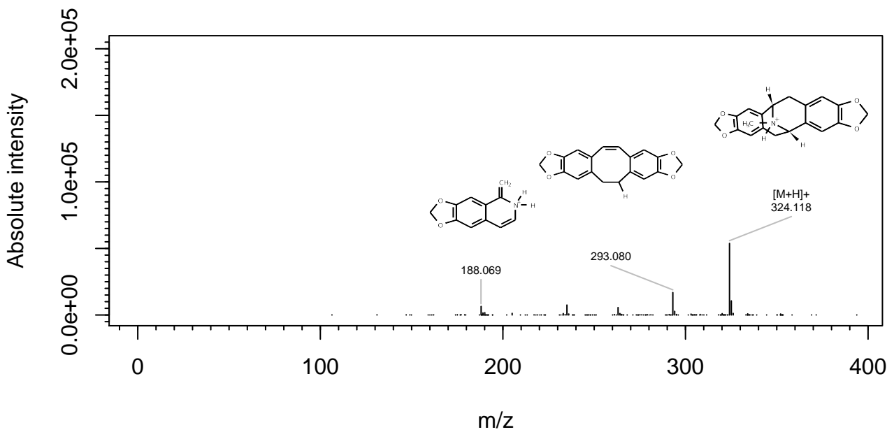
Figure A4. Challenge 4: annotated merged MS/MS spectra of escholtzine (ESI, positive mode).
