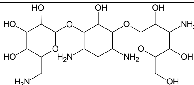
Figure B15. Structures and identifiers for LC-HRMS Challenges 1–4.
