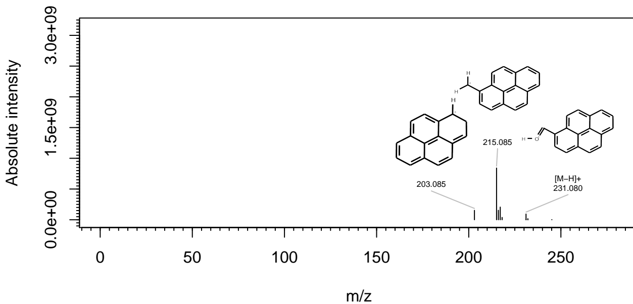
Figure A8. Challenge 11: annotated merged MS and MS/MS spectra of 1-pyrenemethanol (APCI, positive mode).
