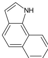
Figure B17. Structures and identifiers for LC-HRMS Challenges 14–17.
