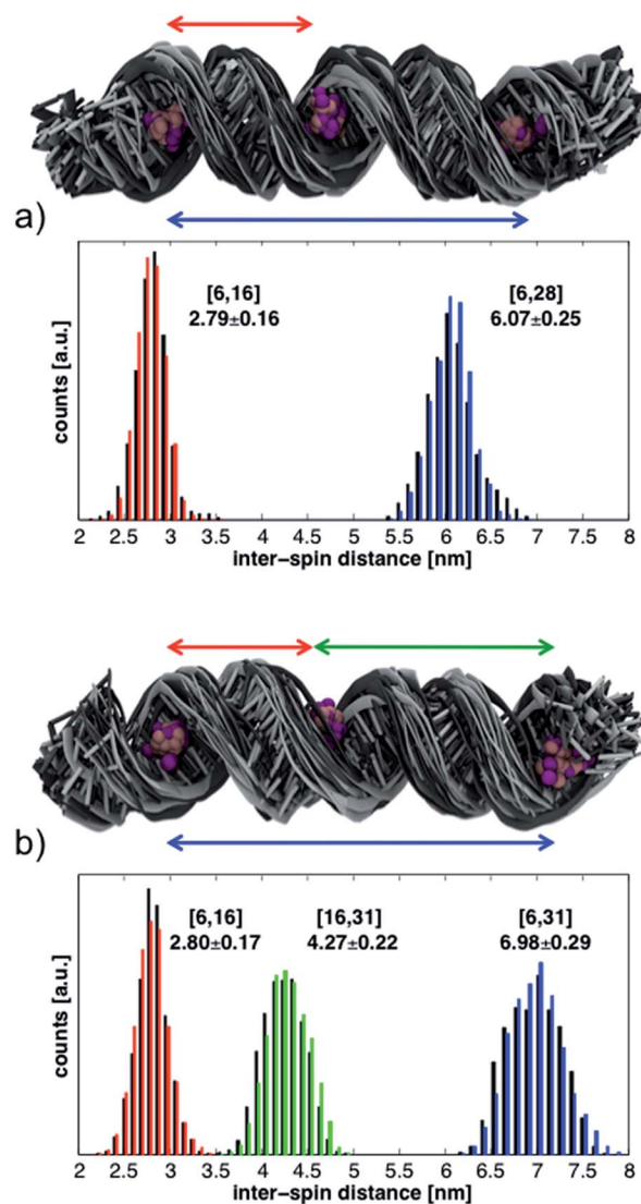
Fig. 6 Structural ensembles and histograms of the inter-spin distances from the MD simulations of RNA helices labeled at positions (a) 6-16-28 and (b) 6-16-31. Structures and histograms from the first 17 ns are shown in black; those from the last 17 ns are in gray or in color. The N and O atoms of the TEMPO moiety are shown with purple (first 17 ns) and pink (last 17 ns) balls. The reported average distances and their standard deviations (in nm) are calculated from the entire 34 ns simulations.
