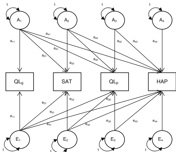
Fig. 2 Cholesky Decomposition for the four measures of SWB for a single person Squares represent measured variables, and circles represent latent, unobserved factors. A represents additive genetic effects, and E is unique environment. Their influence on the phenotype is given by path coefficients a and e . For sake of clarity, the D component is left out of the picture. QL g = Quality of Life in General; SAT = Satisfaction with life; QL p = Quality of life at present; HAP = Subjective Happiness
