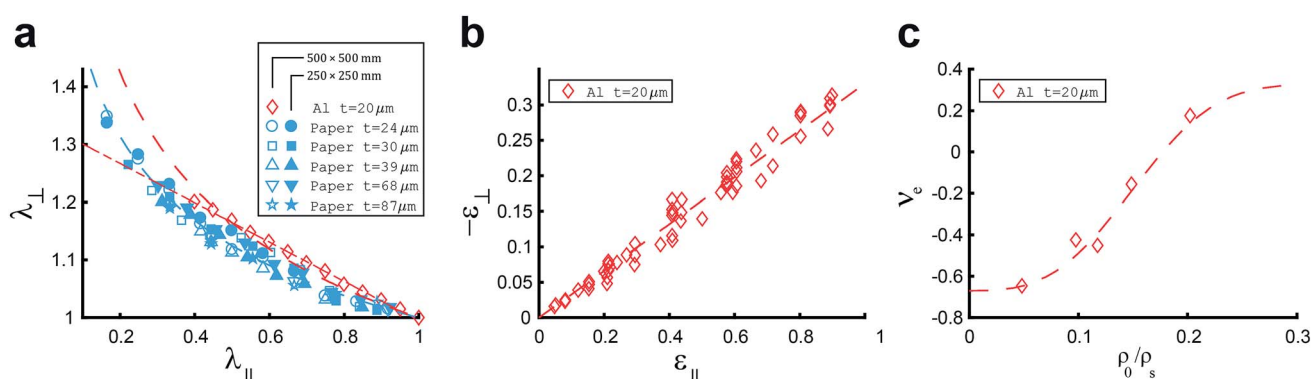
Fig. 4 (a) Lateral expansion ratio ( \lambda_{\perp} ) as a function of axial compression ratio ( \lambda_{\parallel} ) for crumpled aluminium sheets (red diamonds) of initial size 500 \times 500\ \text{mm} , fitted by eqn (20) with \nu = 0.22 (red dashed line) and eqn (19) with \nu_e = 0.34 (red dash-dot line), and for crumpled paper sheets (blue symbols) of initial size 500 \times 500\ \text{mm} (open symbols) and 250 \times 250\ \text{mm} (closed symbols), fitted by eqn (20) with \nu = 0.17 (blue dashed line). (b) Lateral strains ( -\varepsilon_{\perp} ) versus axial strains ( \varepsilon_{\parallel} ) for crumpled aluminum sheets (red diamonds) of thickness t = 20\ \mu\text{m} and initial size 500 \times 500\ \text{mm} and 200 \times 200\ \text{mm} , approximated by eqn (19) with \nu_e = 0.33 (red dashed line). 27 (c) The correlation between the Poisson ratio ( \nu_e ) and the relative density in crumpled aluminum sheets of thickness t = 20\ \mu\text{m} and different initial sizes to create different relative densities, fitted by \nu_e = 0.33 - \exp(-200(\rho_0/\rho_s)^3) . 37
