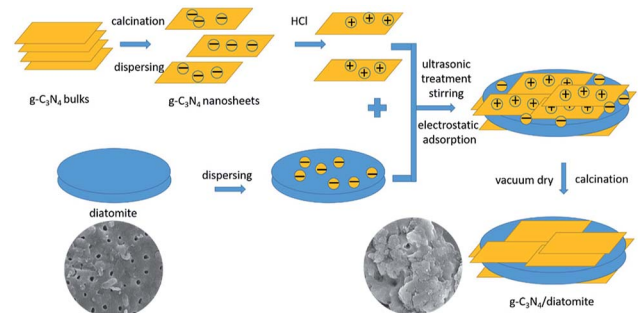
Scheme 1 Synthesis process of g\text{-C}_3\text{N}_4 /diatomite hybrids.
