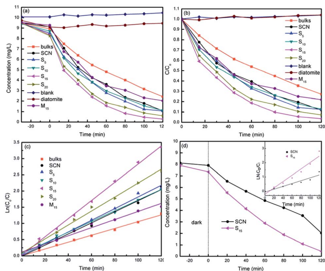
Fig. 10 Concentration change of MO (a) and degradation efficiency of MO (b) during photocatalytic degradation. Linear transform \ln(C_0/C) of the kinetic curves of MO degradation (c), the photocatalytic degradation of phenol (d) and the inset is the linear transform \ln(C_0/C) of the kinetic curves of phenol degradation.
