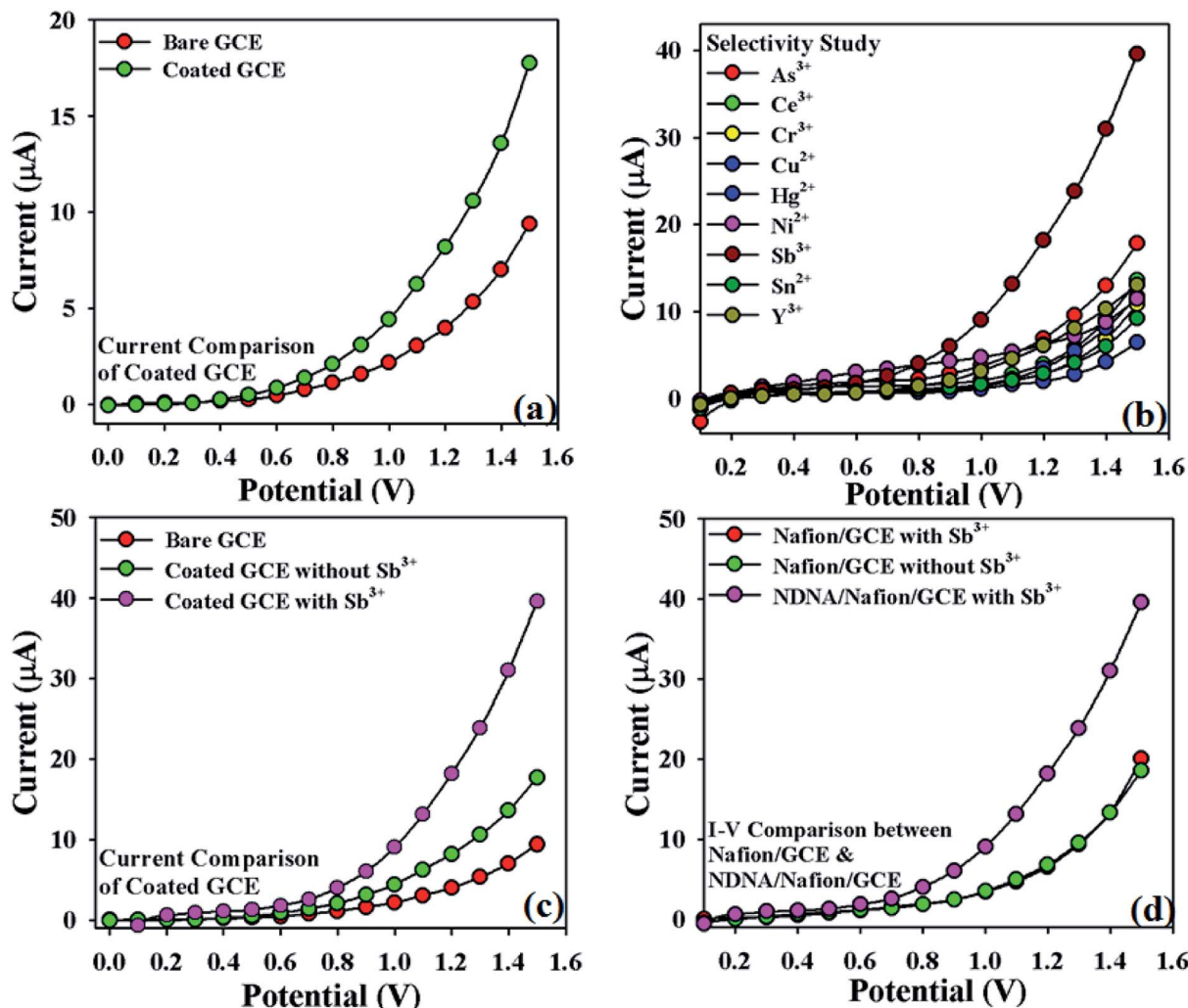
Fig. 3 Selectivity study: (a) I-V response of bare and NDNA-coated GCE; (b) I-V response with various analytes (showing affinity with \text{Sb}^{3+} ), concentration of each analyte was taken at 0.1 \mu\text{M} , 25 \mu\text{L} ; (c) comparison of I-V response of bare and NDNA/nafion/GCE with and without the target analyte \text{Sb}^{3+} at 0.1 \mu\text{M} , 25 \mu\text{L} ; (d) comparison of I-V response of nafion/GCE and NDNA/nafion/GCE with and without the target analyte.
