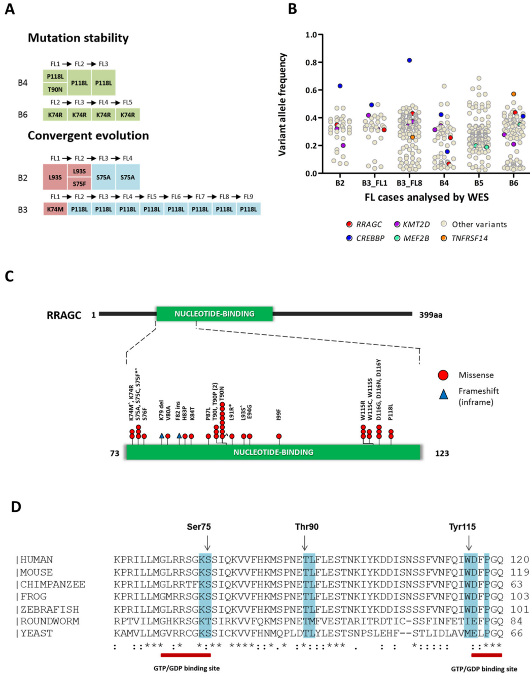
Figure 1. Identification of frequent RRAGC mutations in FL. (a) RRAGC mutations show two different patterns of conservation in successive tumor biopsies during FL progression in the discovery WES cases: mutation stability and convergent evolution. (b) Variant allele frequency (VAF) distribution and density for all the non-synonymous mutations identified in the 5 WES cases. In each case, the first available biopsy is depicted, with the exception of B3 where two time points are illustrated (B3_FL1 and B3_FL8). (c) Schema of the protein domain and locations of the RRAGC mutations identified in this study (NCBI protein
