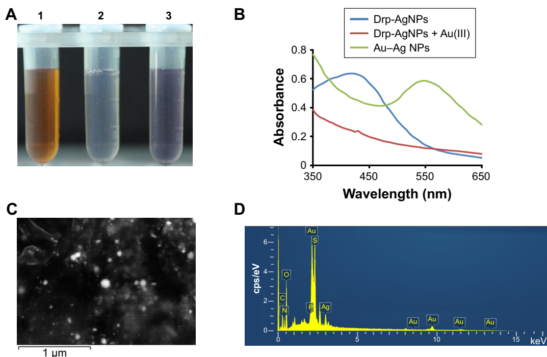
Figure 9 Synthesis of Au–Ag bimetallic NPs based on Drp-AgNPs.
